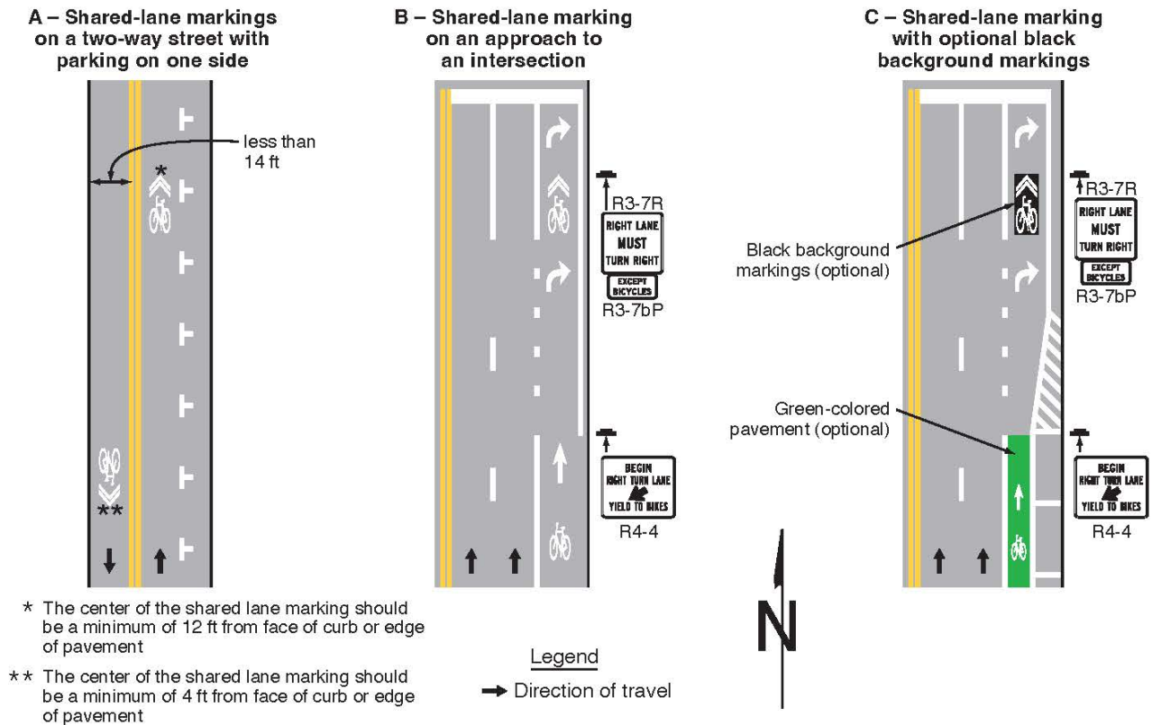
Figure 9E-9. Examples of Shared-Lane Marking Applications
