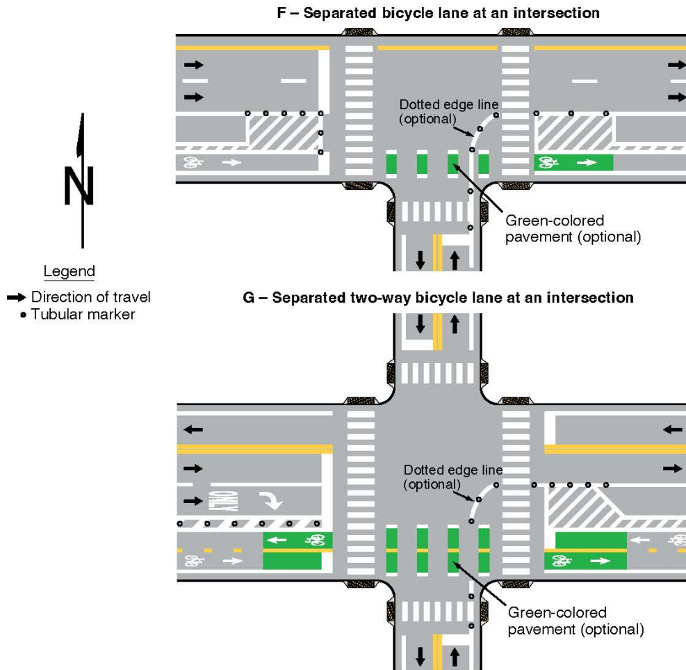
Figure 9E-7. Examples of Lane Markings for Separated Bicycle Lanes (Sheet 2 of 2)
