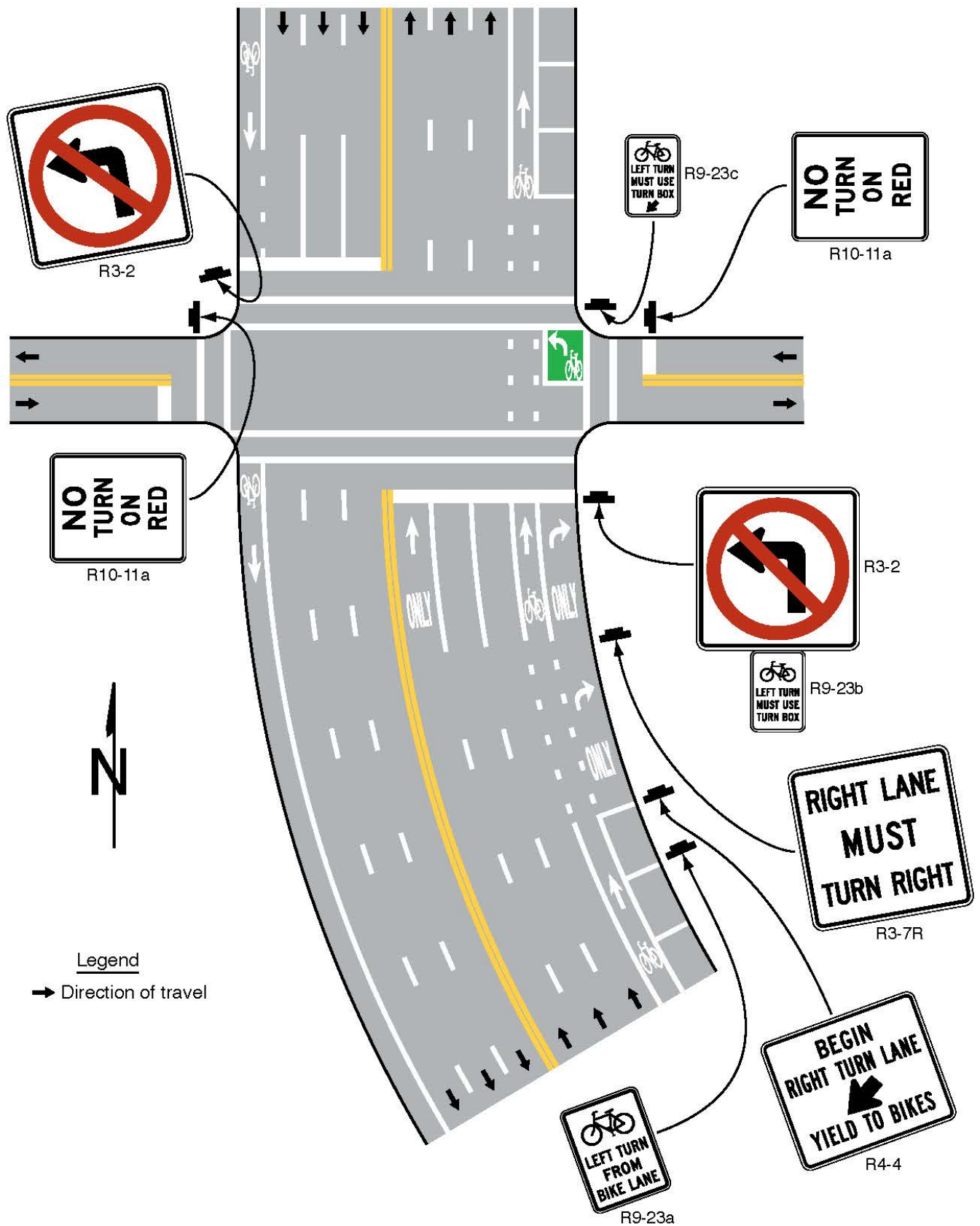
Figure 9B-5. Example of Two-Stage Bicycle Turn Box where Use is Mandatory
