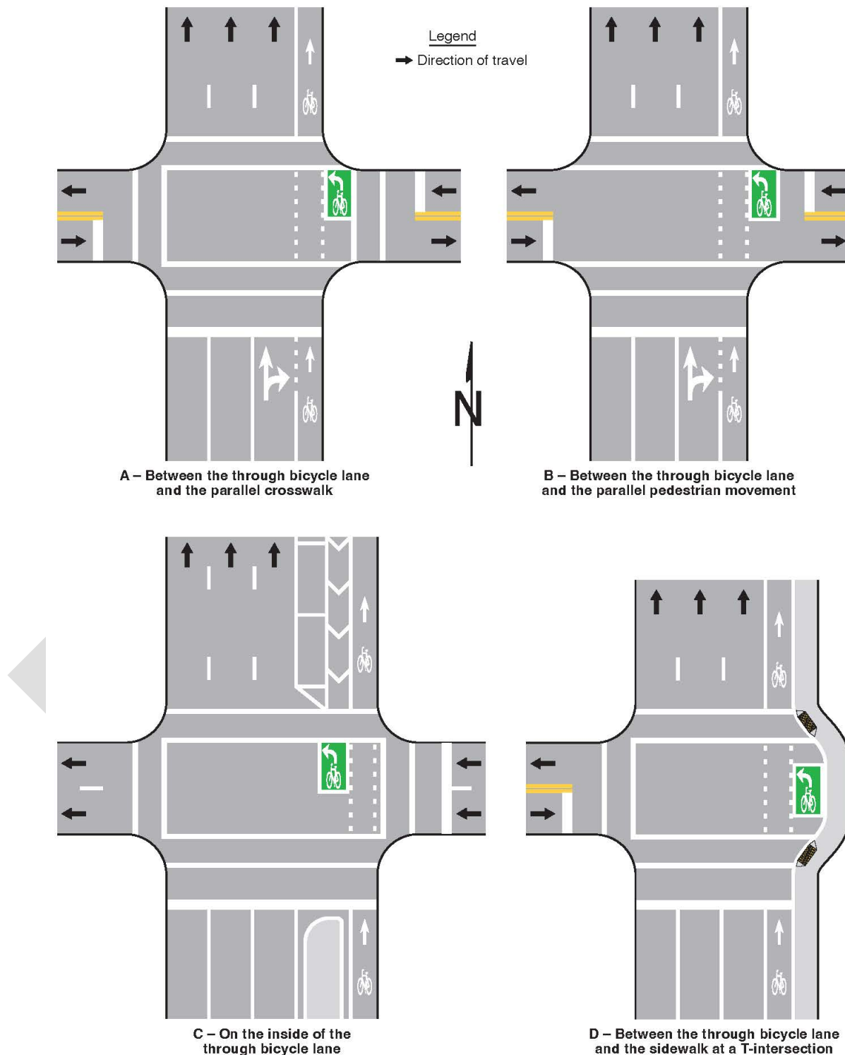
Figure 9E-10. Examples of Two-Stage Turn Box Locations at Intersections
