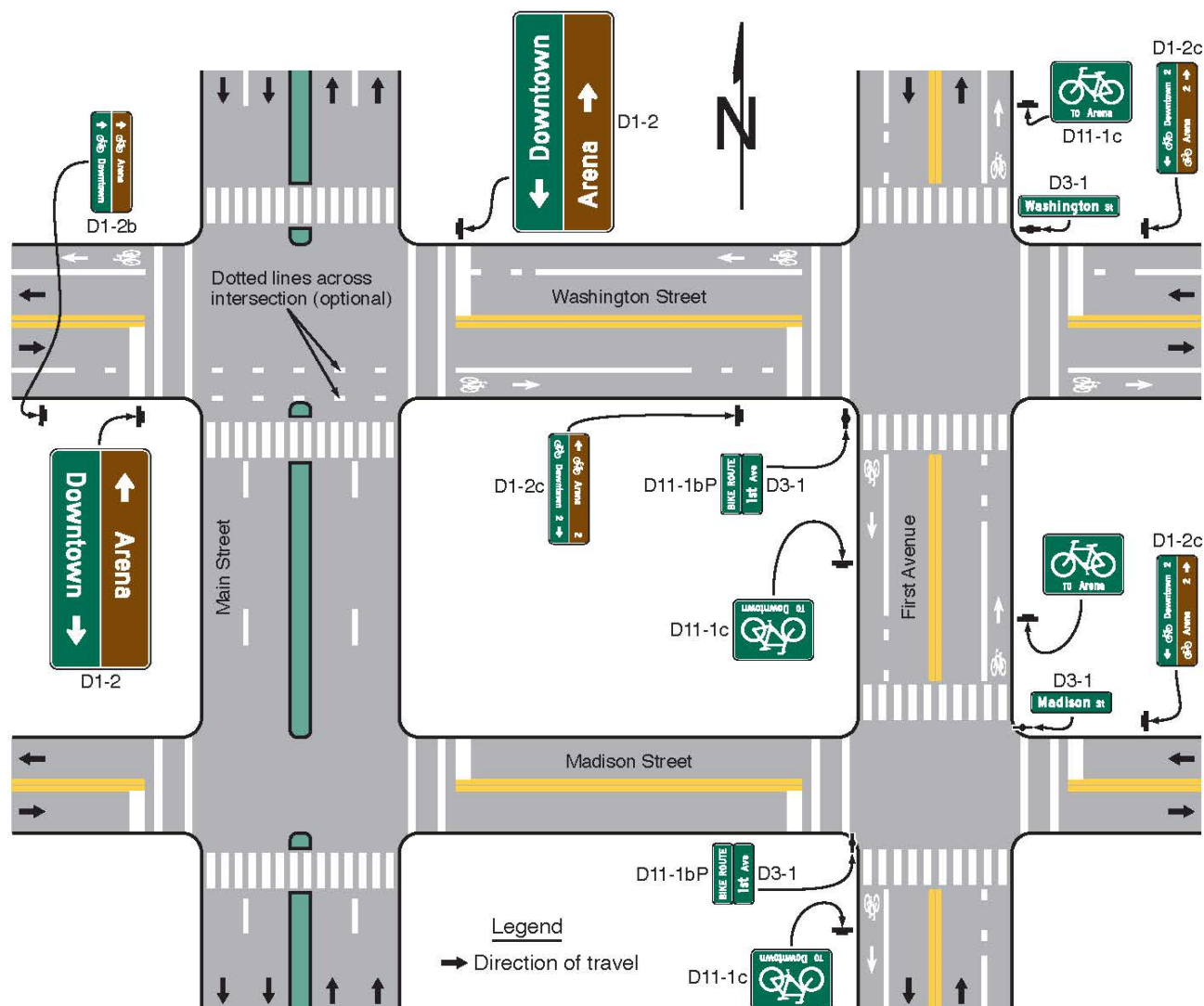
Figure 9D-3. Example of Bicycle Route Guide Signing
