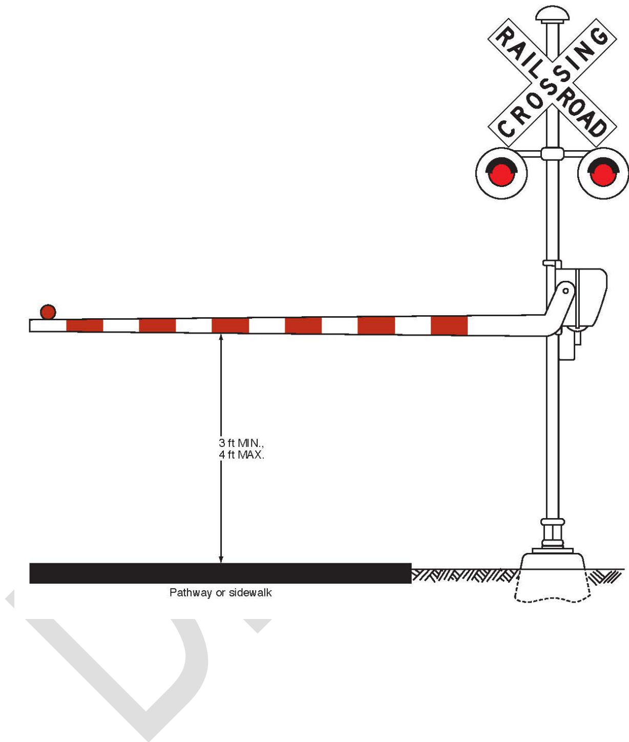
Figure 8E-8. Example of an Automatic Pedestrian Gate at a Pathway or Sidewalk Grade Crossing
