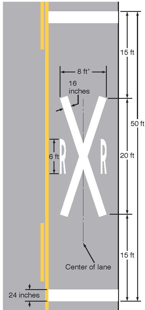
A – Grade crossing pavement marking symbol
