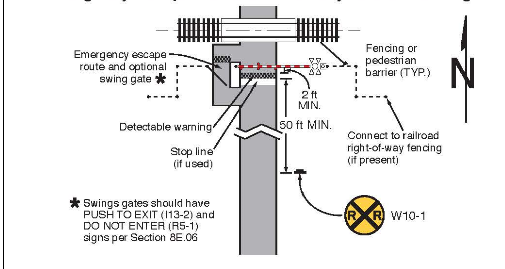
Figure 8E-6. Example of an Automatic Pedestrian Gate and an Emergency Escape Route at a Pathway Grade Crossing
