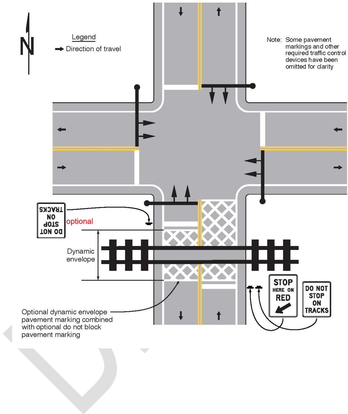
Figure 8C-4. Example of Dynamic Envelope and Do Not Block Pavement Markings at Grade Crossings
