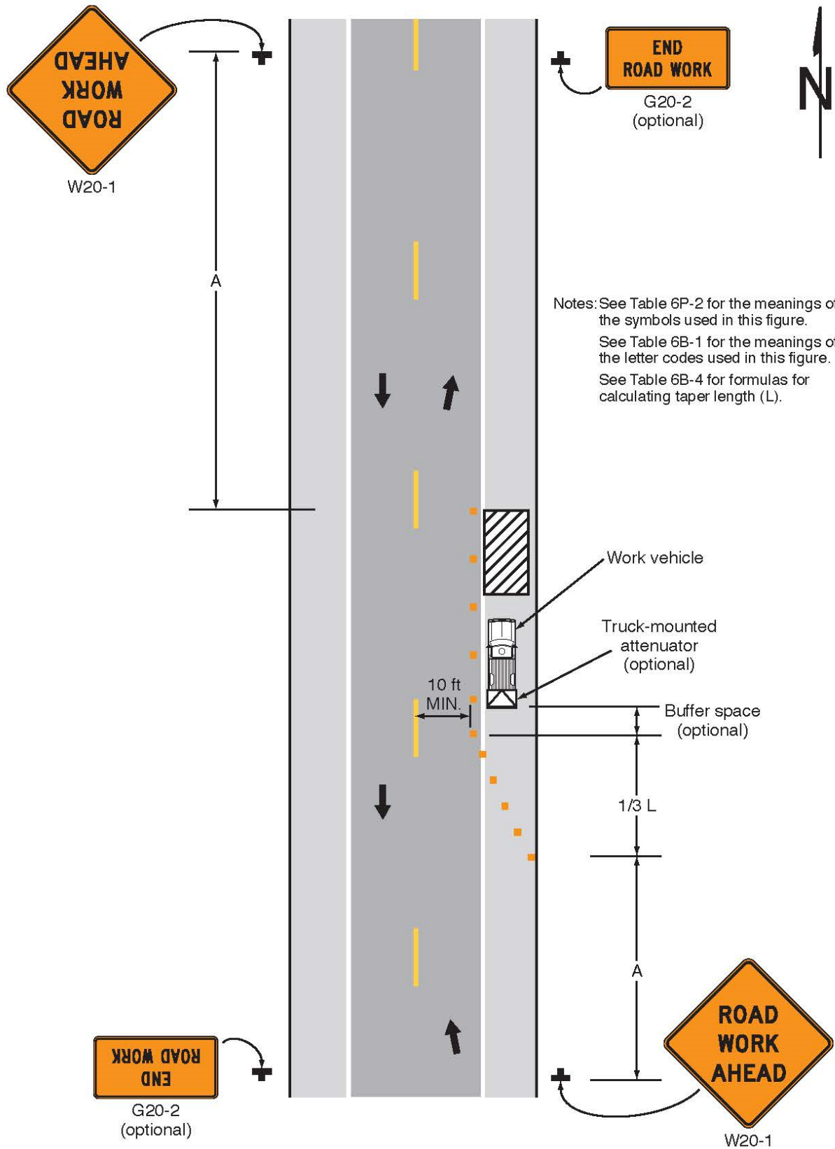
Figure 6P-6. Shoulder Work with Minor Encroachment (TA-6)
