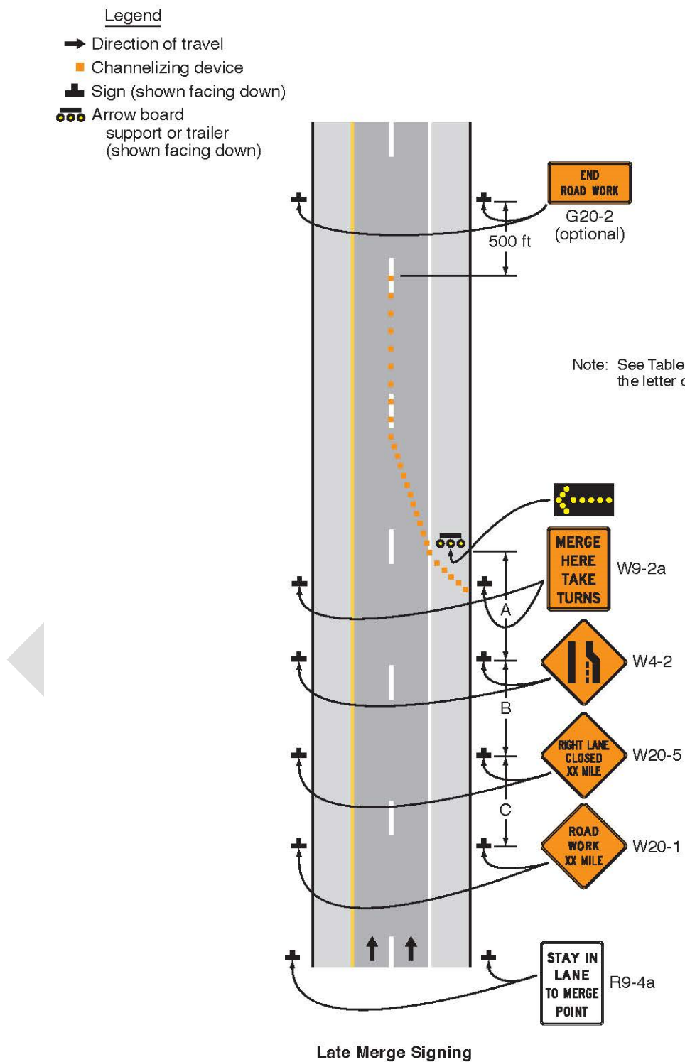
Figure 6N-1. Late Merge
