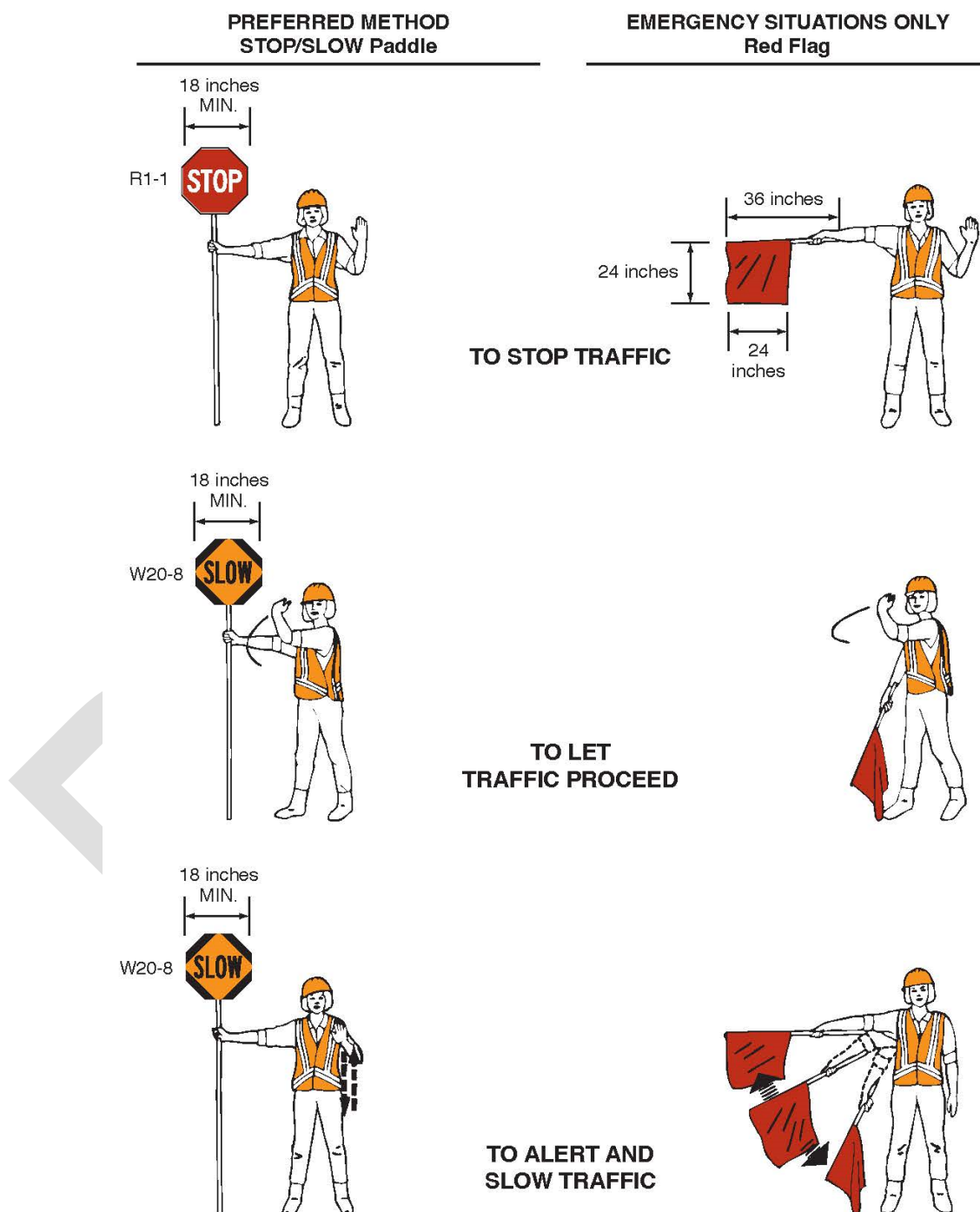
Figure 6D-1. Use of Hand-Signaling Devices by Flaggers
