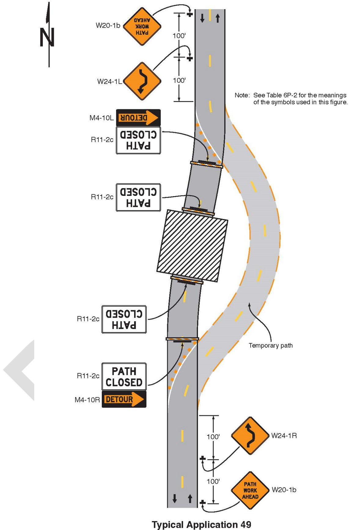
Figure 6P-49. Shared-Use Path Closure with a Diversion (TA-49)
