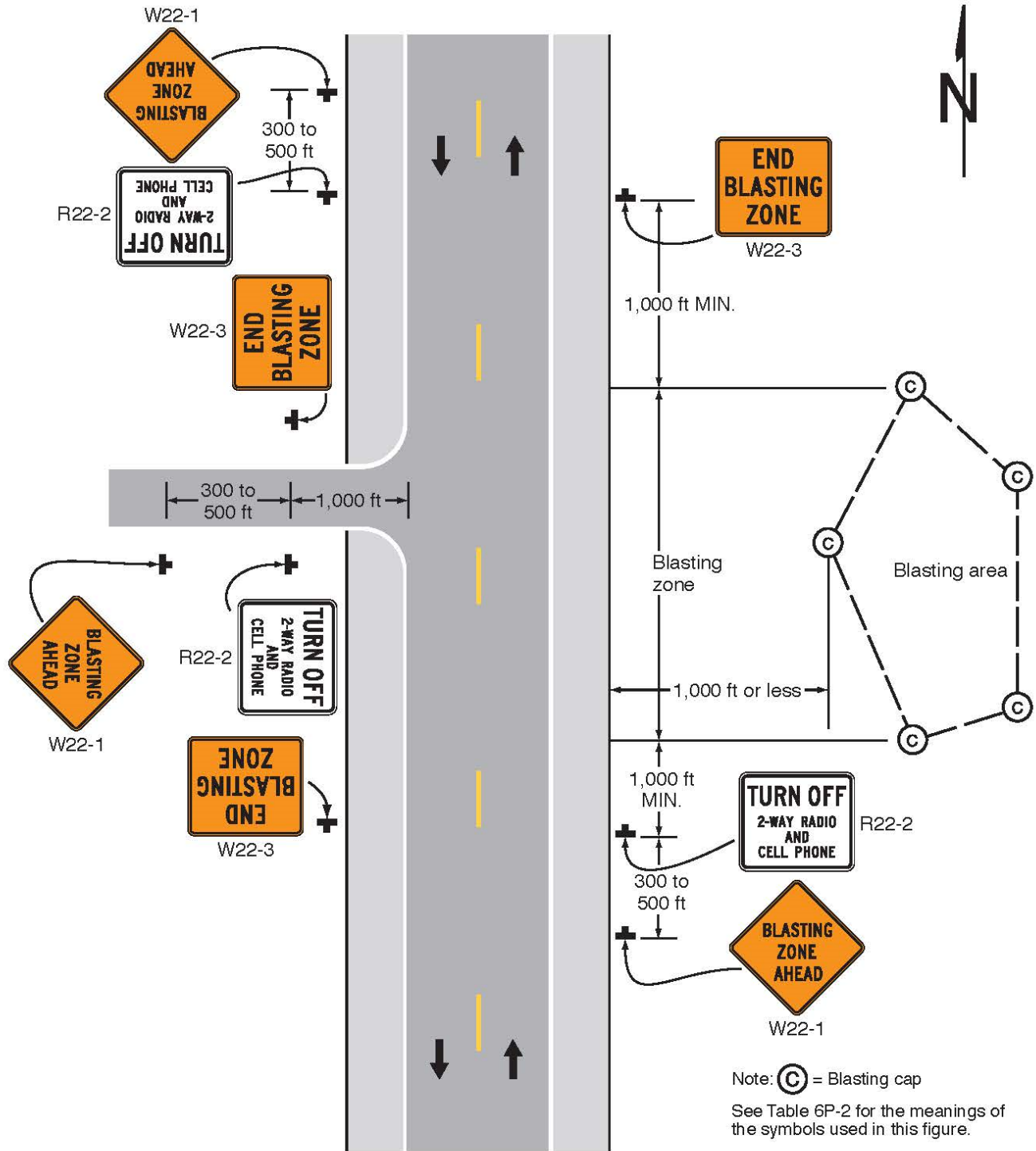
Figure 6P-2. Blasting Zone (TA-2)
