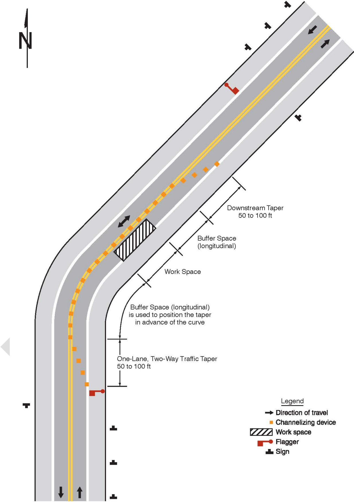
Figure 6B-3. Example of a One-Lane, Two-Way Traffic Taper
