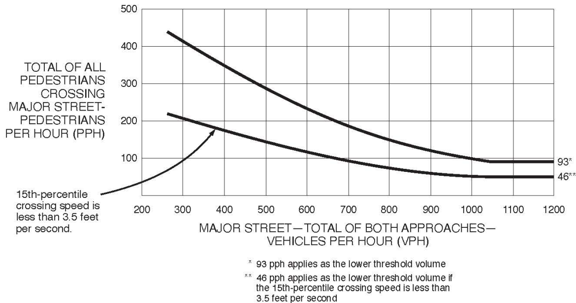
Figure 4C-8. Warrant 4, Pedestrian Peak Hour (70% Factor) (COMMUNITY LESS THAN 10,000 POPULATION OR ABOVE 35 MPH ON MAJOR STREET)
