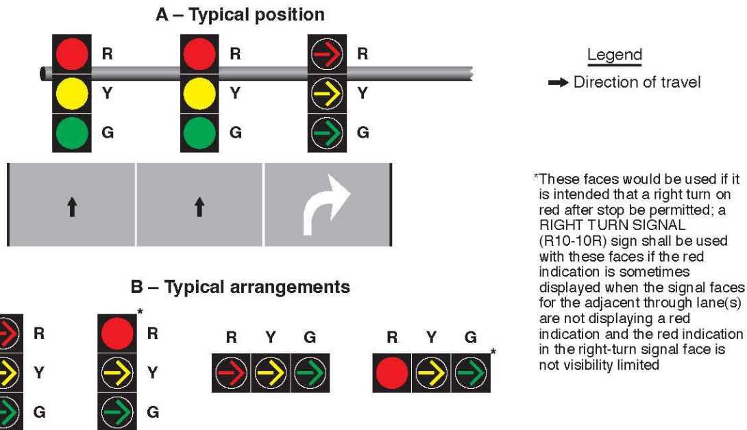
Figure 4F-12. Typical Position and Arrangements of Separate Signal Faces for Protected Only Mode Right Turns
