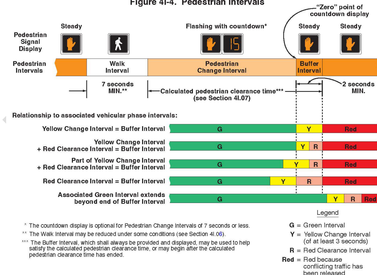
Figure 4I-4. Pedestrian Intervals
