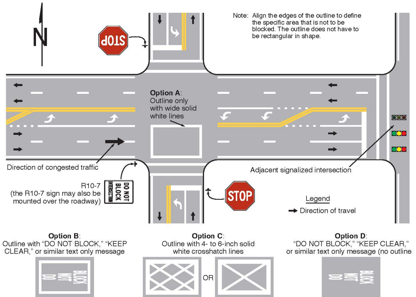
Figure 3B-24. Do Not Block Intersection Markings
