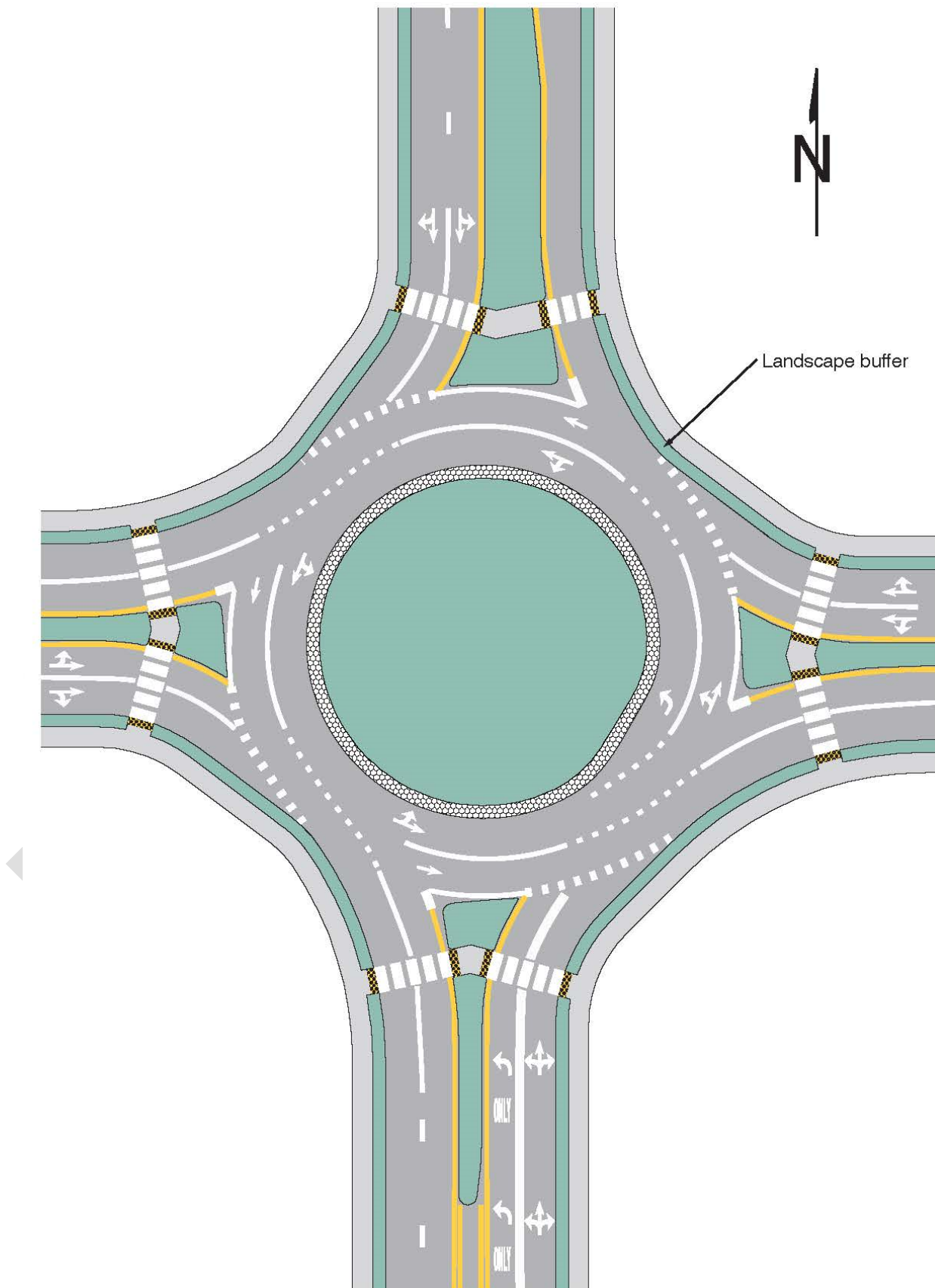
Figure 3D-6. Example of Markings for a Two-Lane Roundabout with a Double Left Turn
