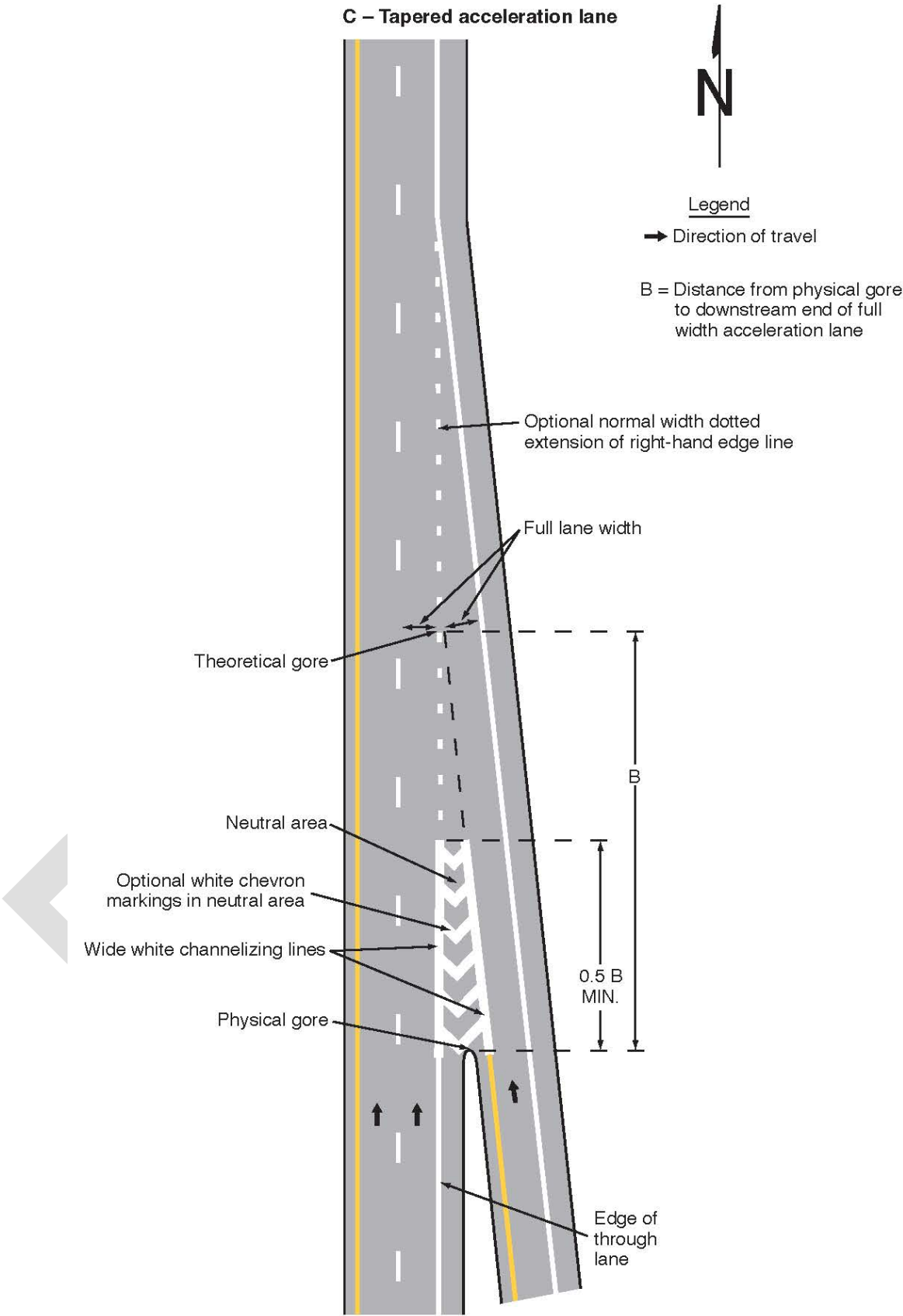
Figure 3B-10. Examples of Dotted Line and Channelizing Line Applications for Entrance Ramp Markings (Sheet 2 of 2)
