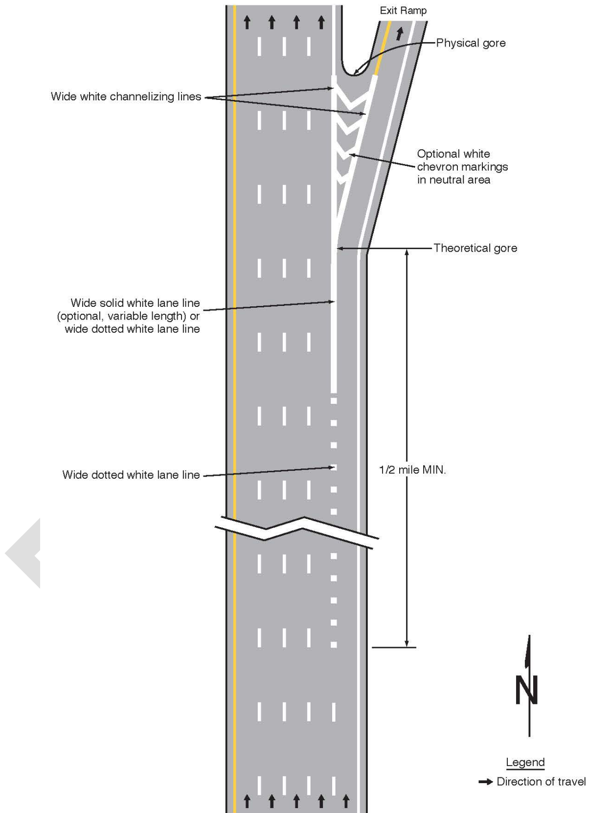
Figure 3B-11. Examples of Applications of Freeway and Expressway Lane-Drop Markings (Sheet 1 of 6)
