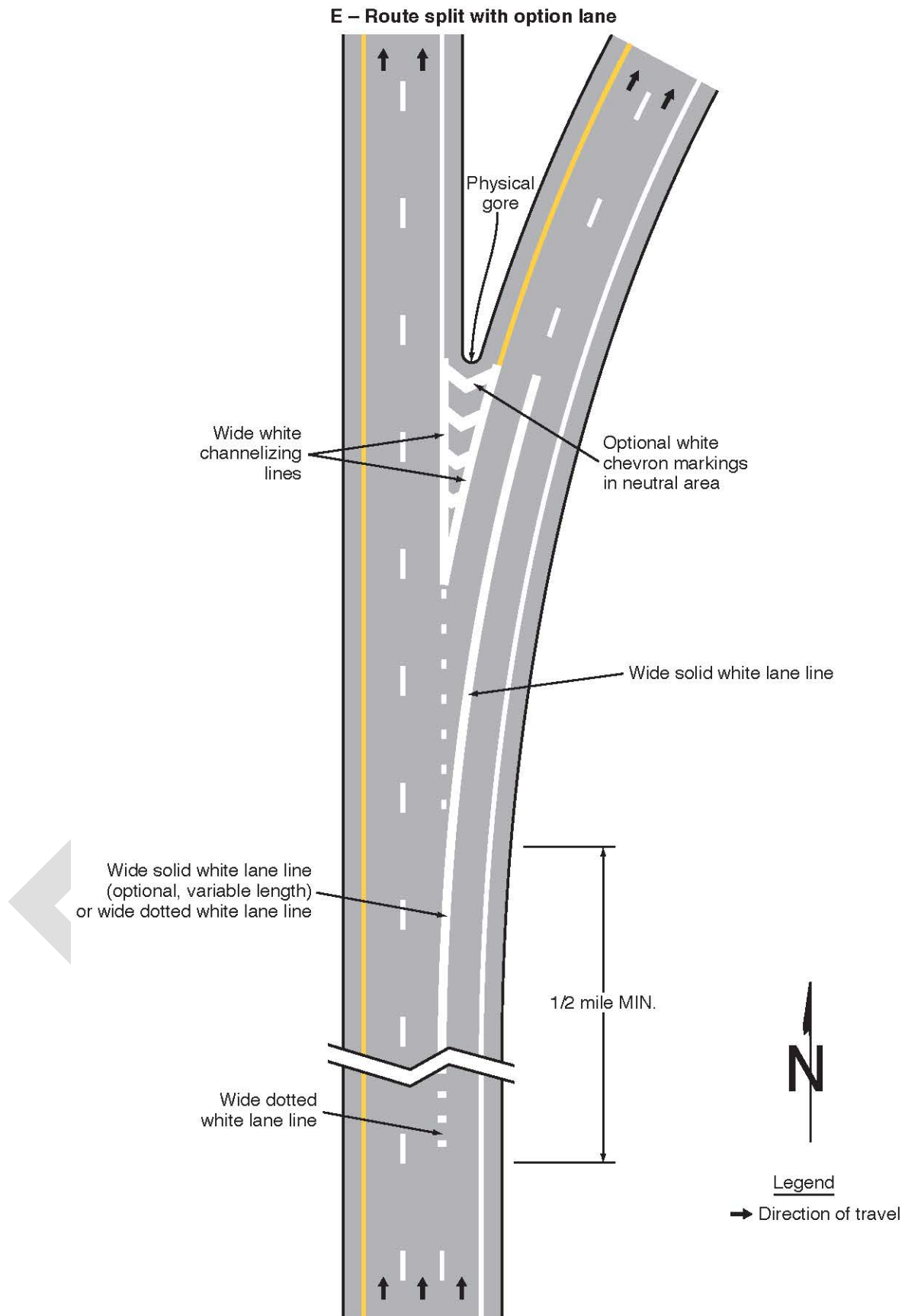
Figure 3B-11. Examples of Applications of Freeway and Expressway Lane-Drop Markings (Sheet 5 of 6)
