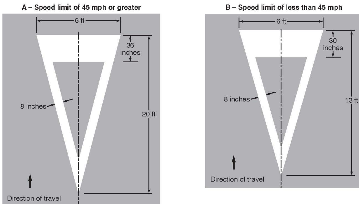
Figure 3B-20. Yield Ahead Triangle Symbols
