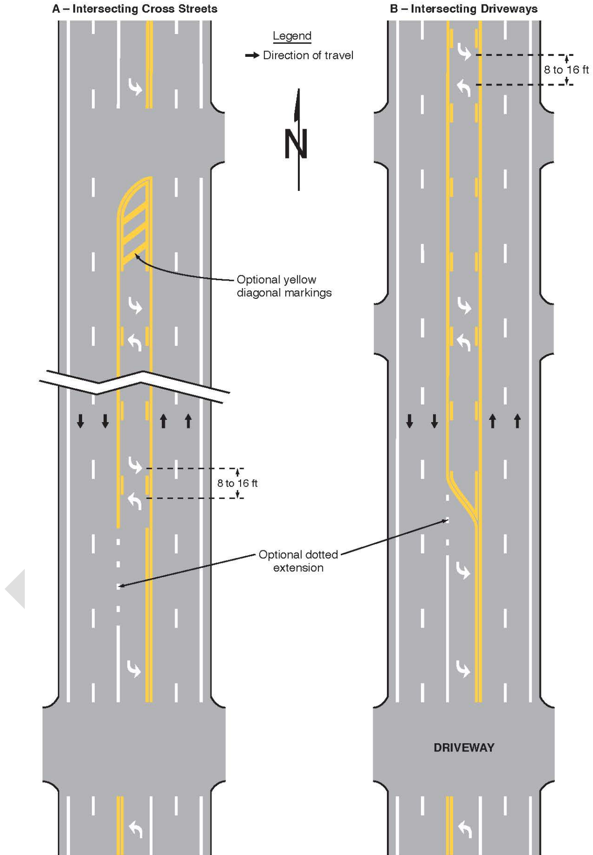
Figure 3B-7. Examples of Two-Way Left-Turn Lane Marking Applications
