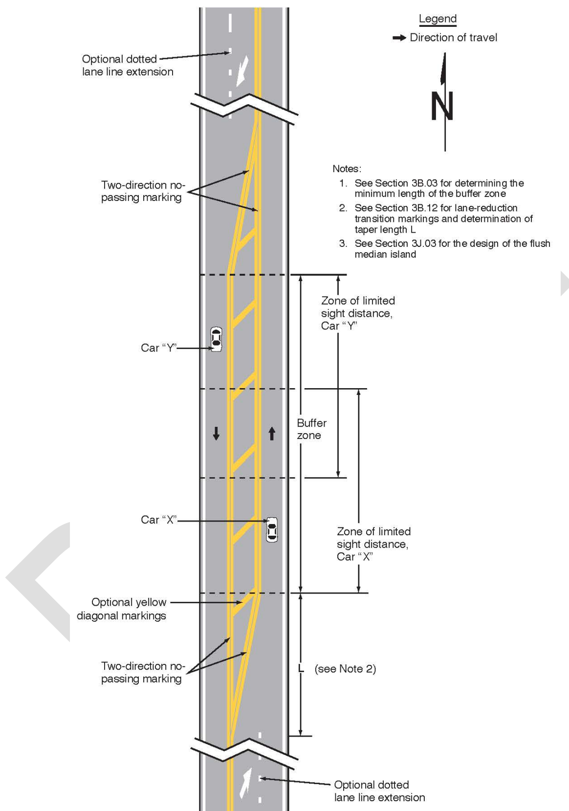
Figure 3B-5. Application of Three-Lane, Two-Way Markings for Changing the Direction of the Center Lane
