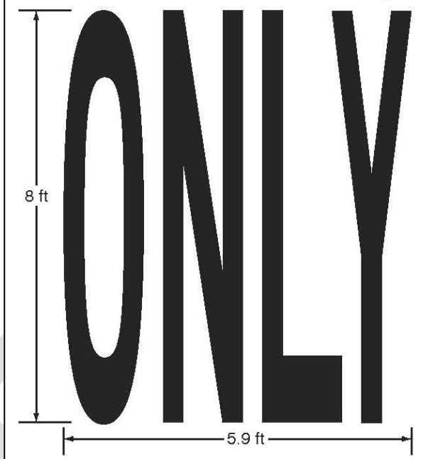
Figure 3B-17. Example of Elongated Letters for Word Pavement Markings
