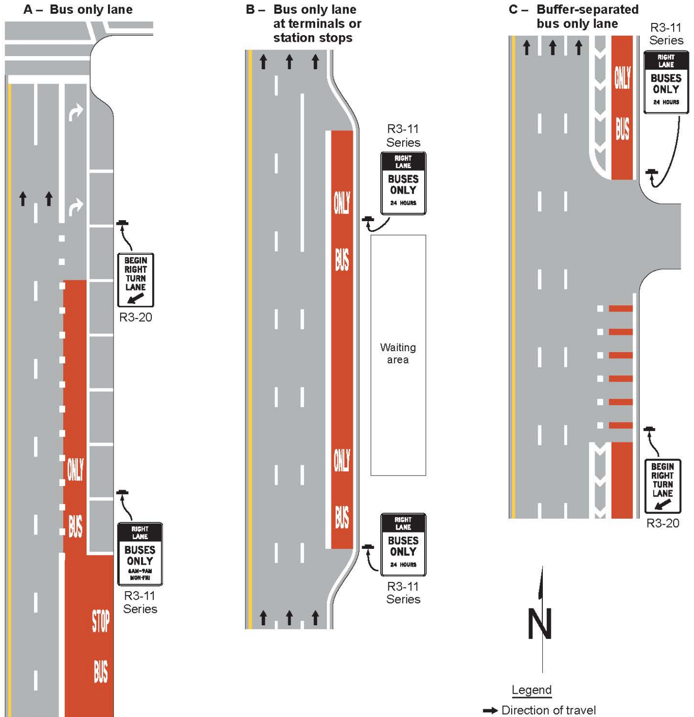
Figure 3H-5. Examples of Red-Colored Pavement Applications
