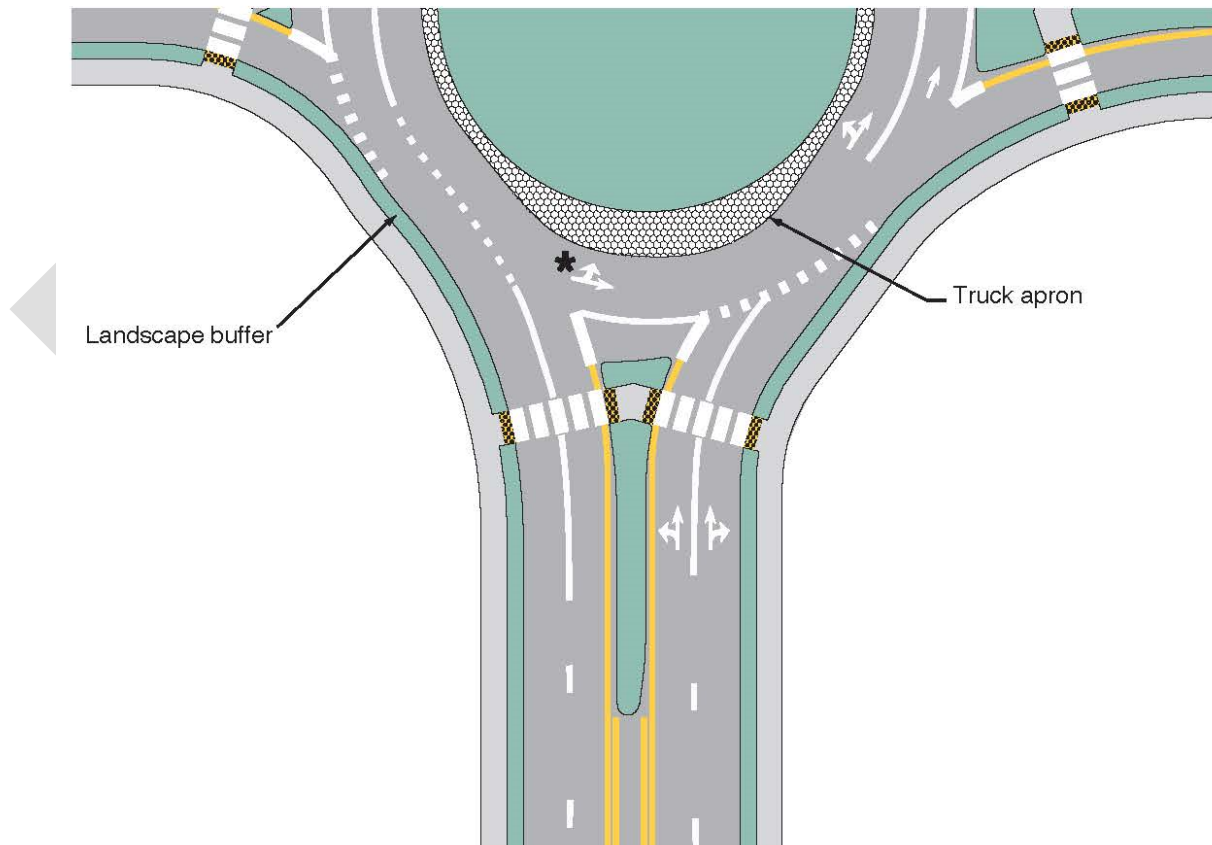
C – Central island extended by a truck apron
