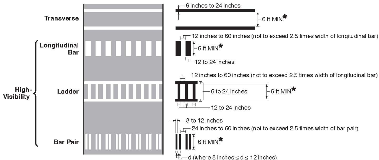
Figure 3C-1. Crosswalk Markings
