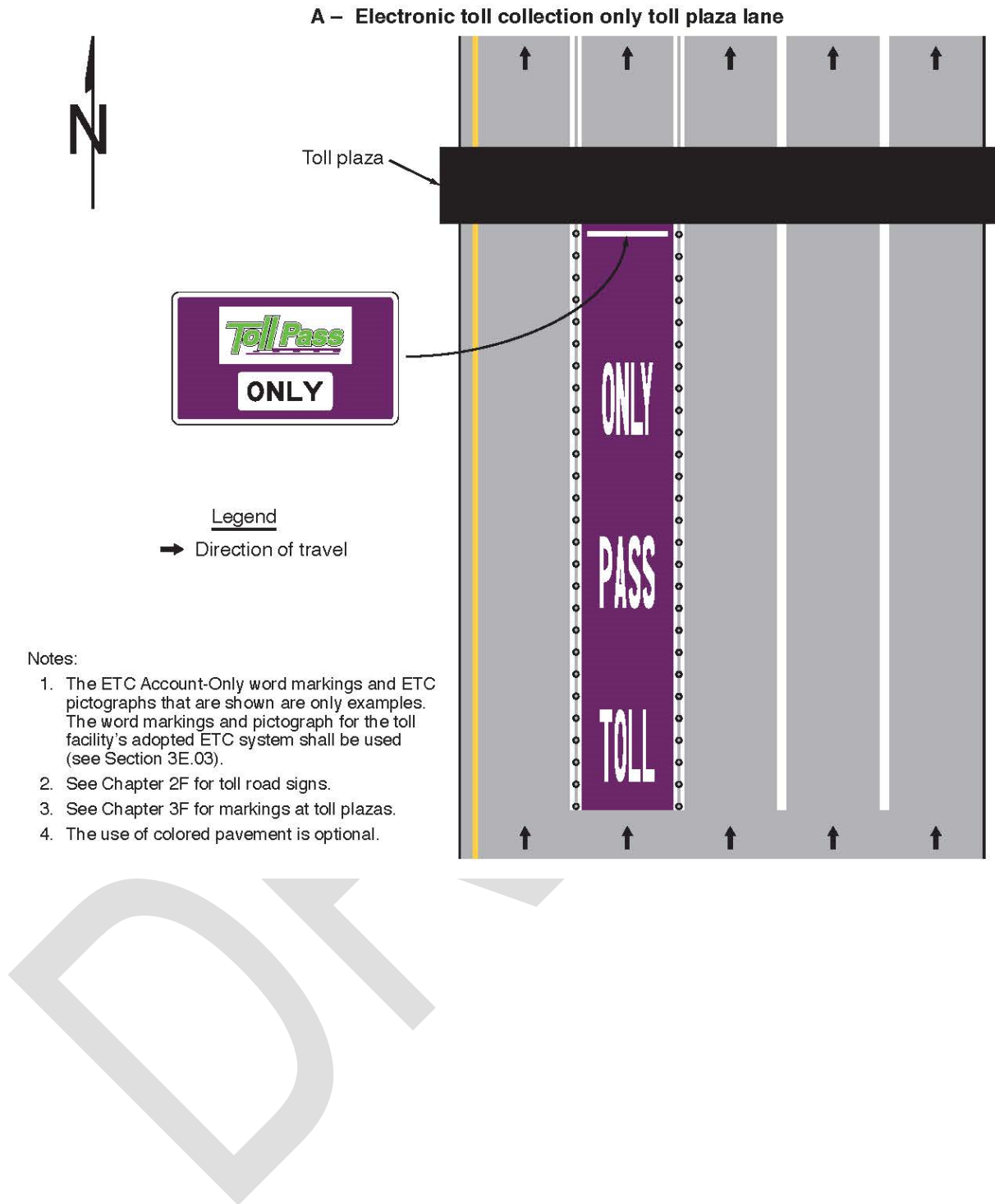
Figure 3H-6. Examples of Purple-Colored Pavement Applications (Sheet 1 of 2)
