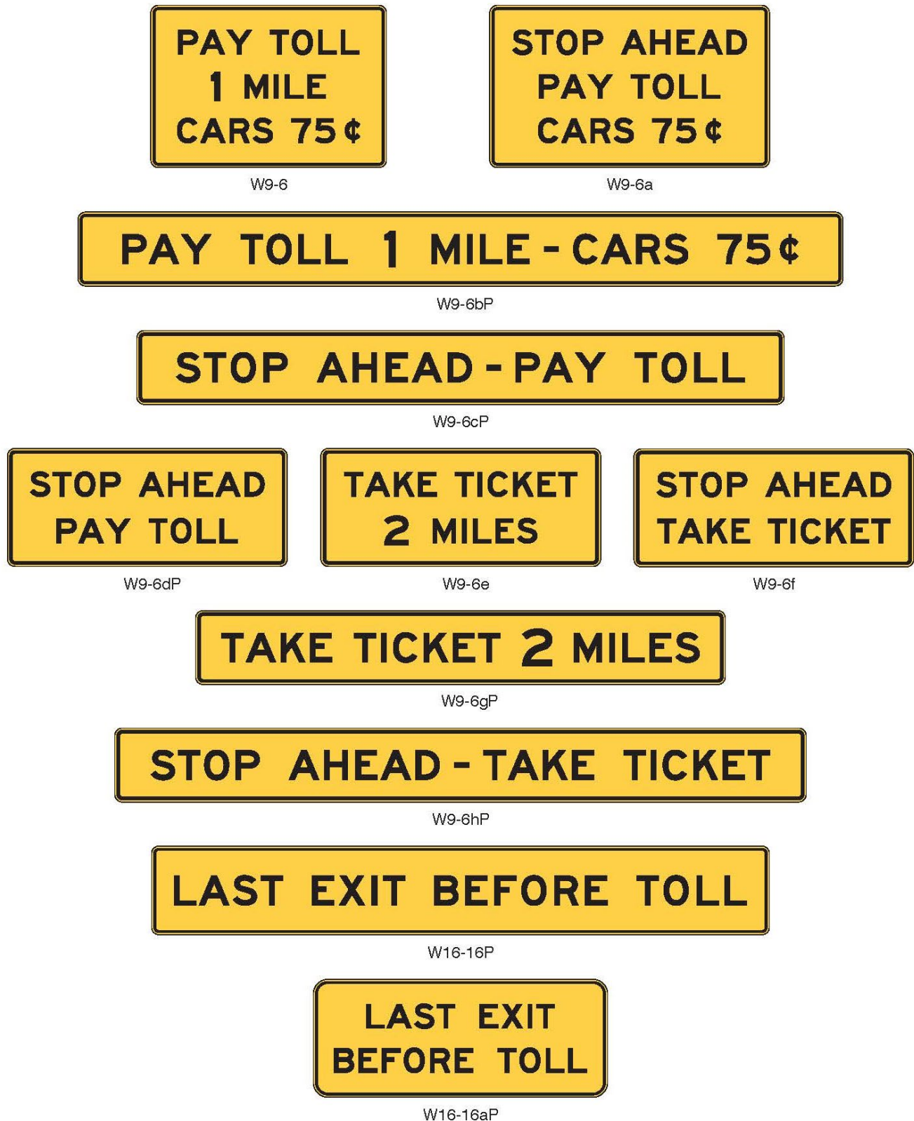
Figure 2F-4. Toll Plaza Warning Signs and Plaques
