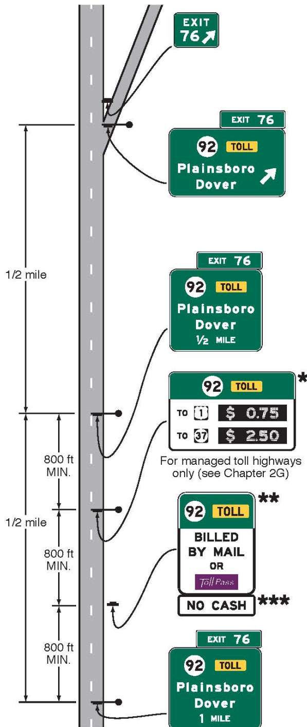
Figure 2F-12. Examples of Guide Signs for the Entrance to a Toll Highway on which Tolls are Collected Electronically Only (Sheet 3 of 3)
