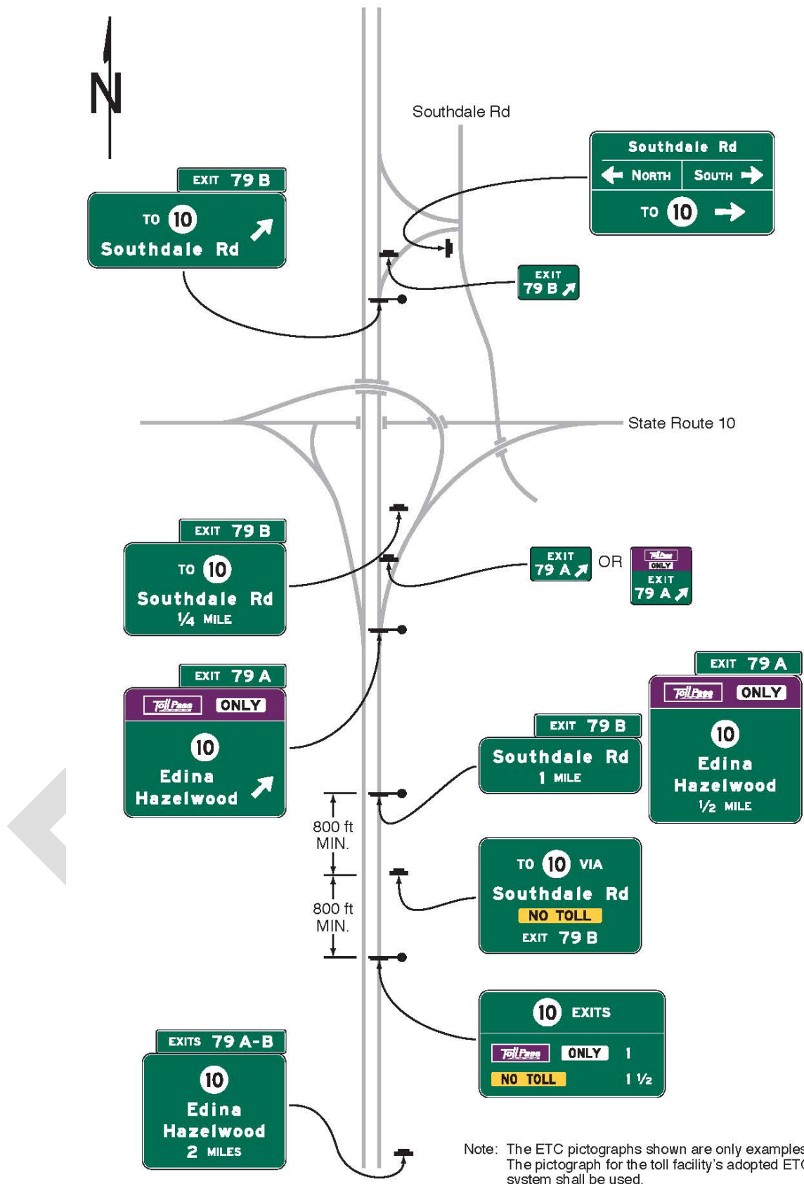
Figure 2F-13. Examples of Guide Signs for Alternative Toll and Non-Toll Ramp Connections to a Non-Toll Highway
