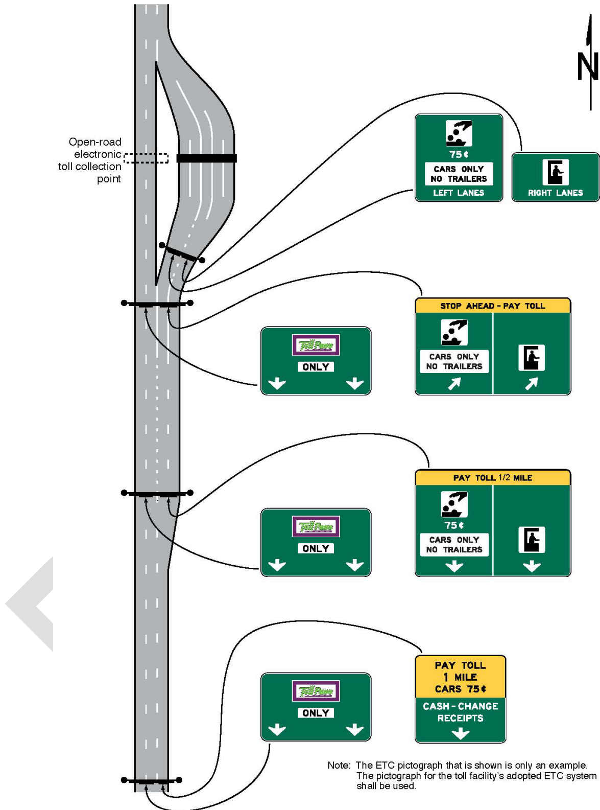
Figure 2F-15. Examples of Guide Signs for a Mainline Toll Plaza on a Diverging Alignment from Open-Road ETC Lanes
