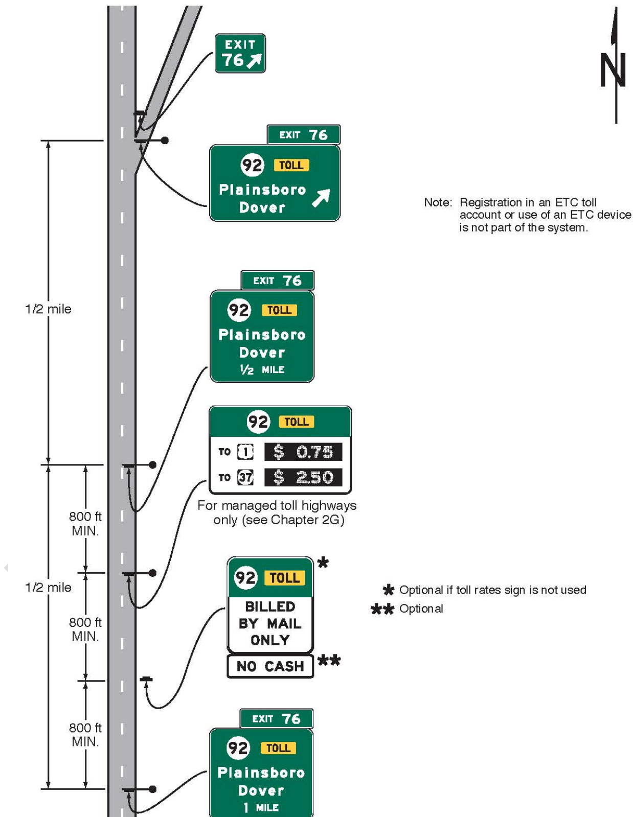
Figure 2F-12. Examples of Guide Signs for the Entrance to a Toll Highway on which Tolls are Collected Electronically Only (Sheet 1 of 3)
