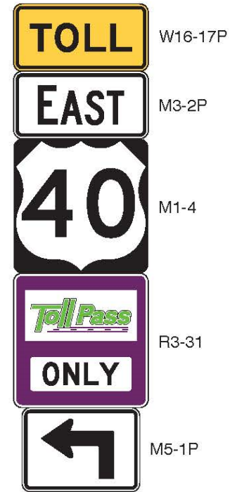
Figure 2F-3. ETC Account-Only Auxiliary Signs for Use in Route Sign Assemblies
