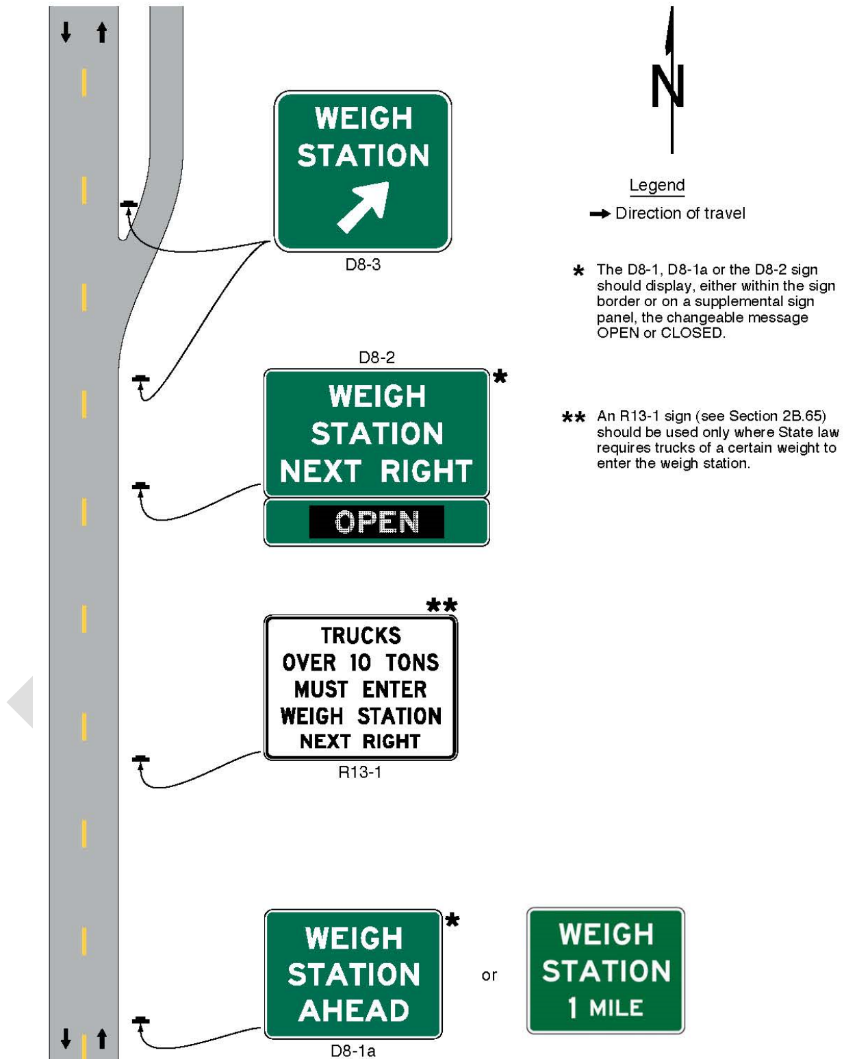
Figure 2D-23. Example of Weigh Station Signing – Conventional Road
