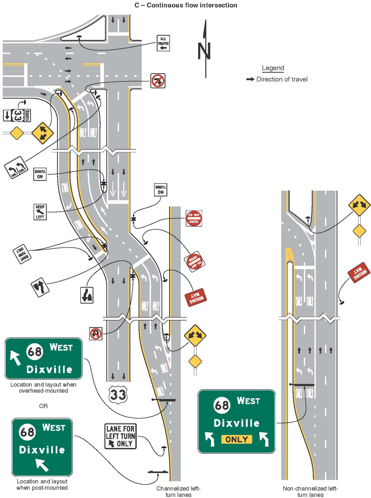
Figure 2D-13. Examples of Signing for Intersections with Indirect Left Turns (Sheet 3 of 3)
