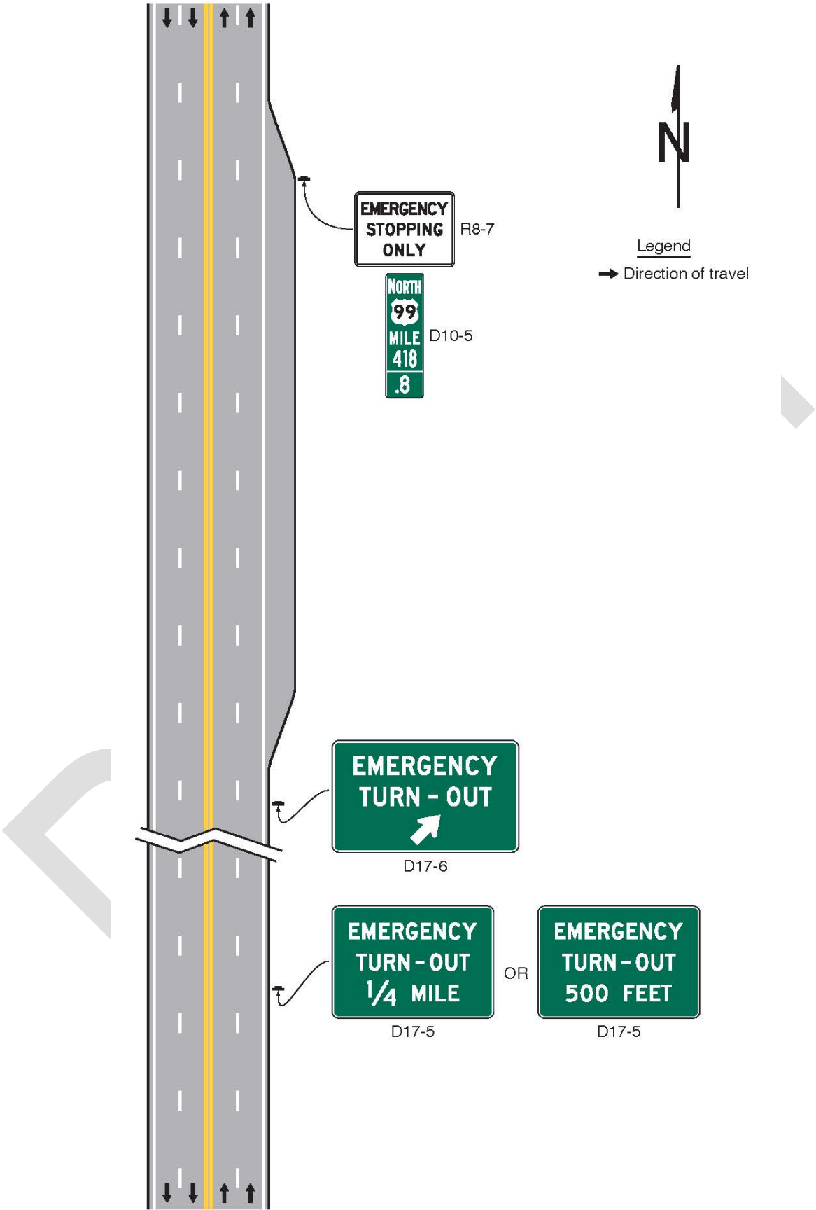
Figure 2D-29. Example of Signing for an Emergency Turn-Out
