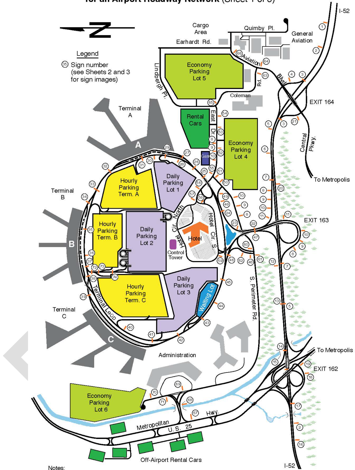
Figure 2D-39. Example of a System of Major Guide Signs for an Airport Roadway Network (Sheet 1 of 3)
