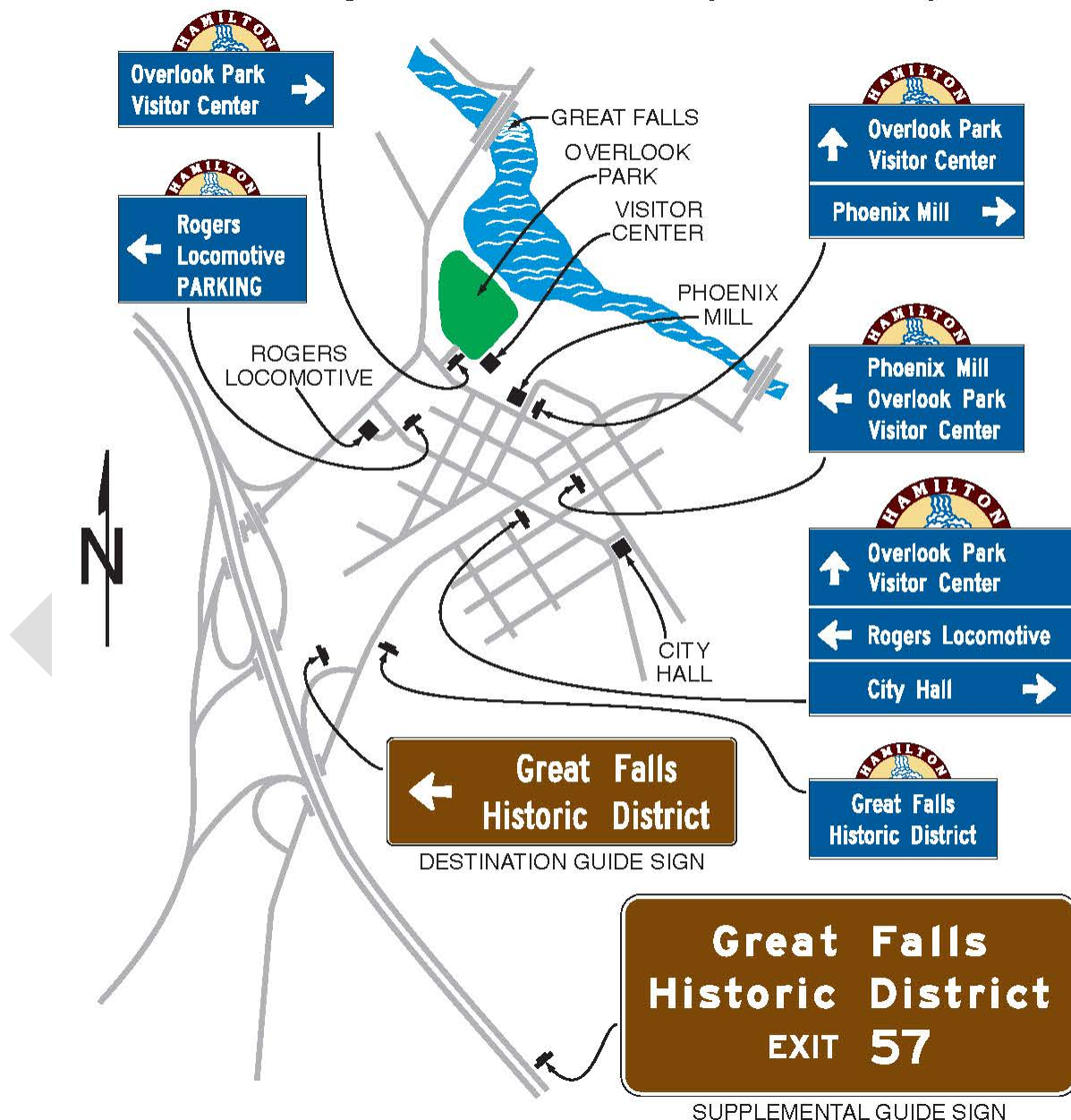
Figure 2D-31. Example of a Community Wayfinding Guide Sign System Showing Direction from a Freeway or Expressway
