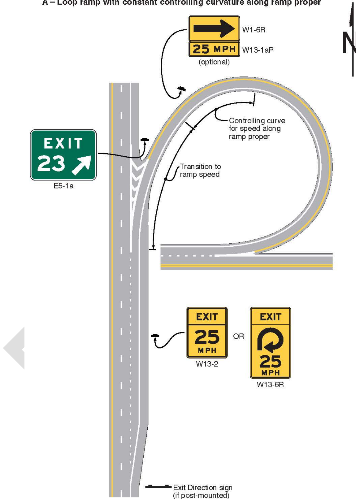
Figure 2C-3. Examples of Exit Ramp Advisory Speed and Other Warning Signs (Sheet 1 of 5)
