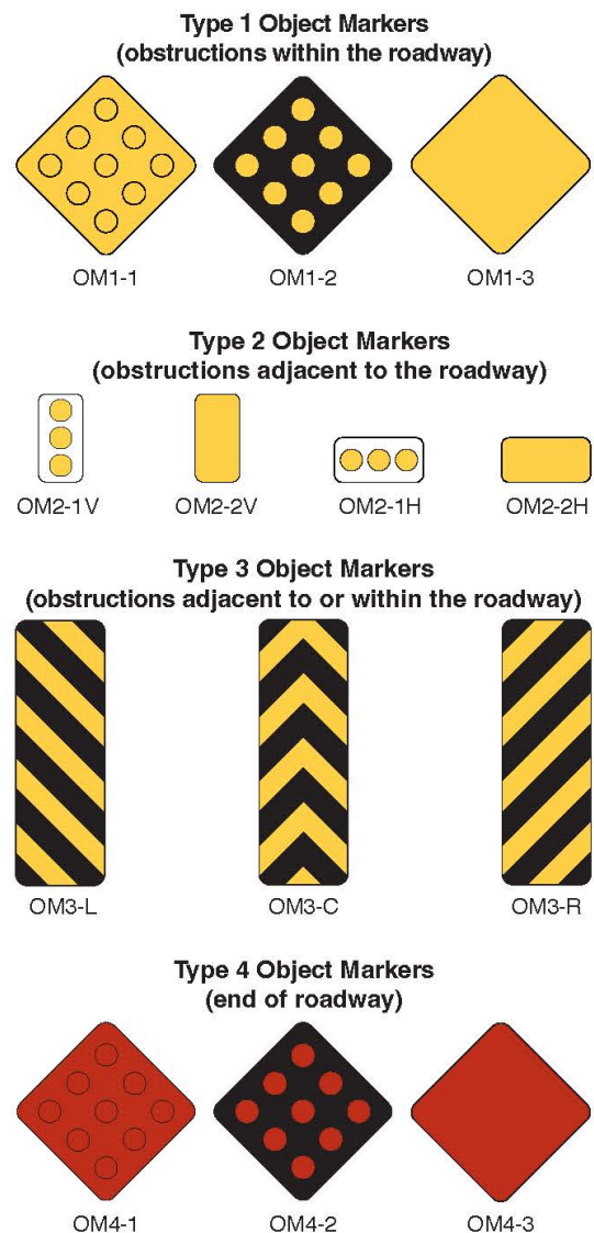
Figure 2C-17. Object Markers
