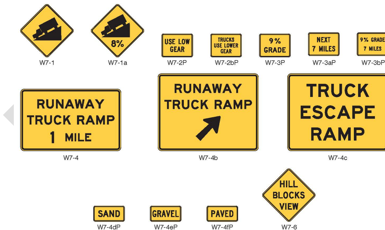
Figure 2C-5. Vertical Grade Signs and Plaques
