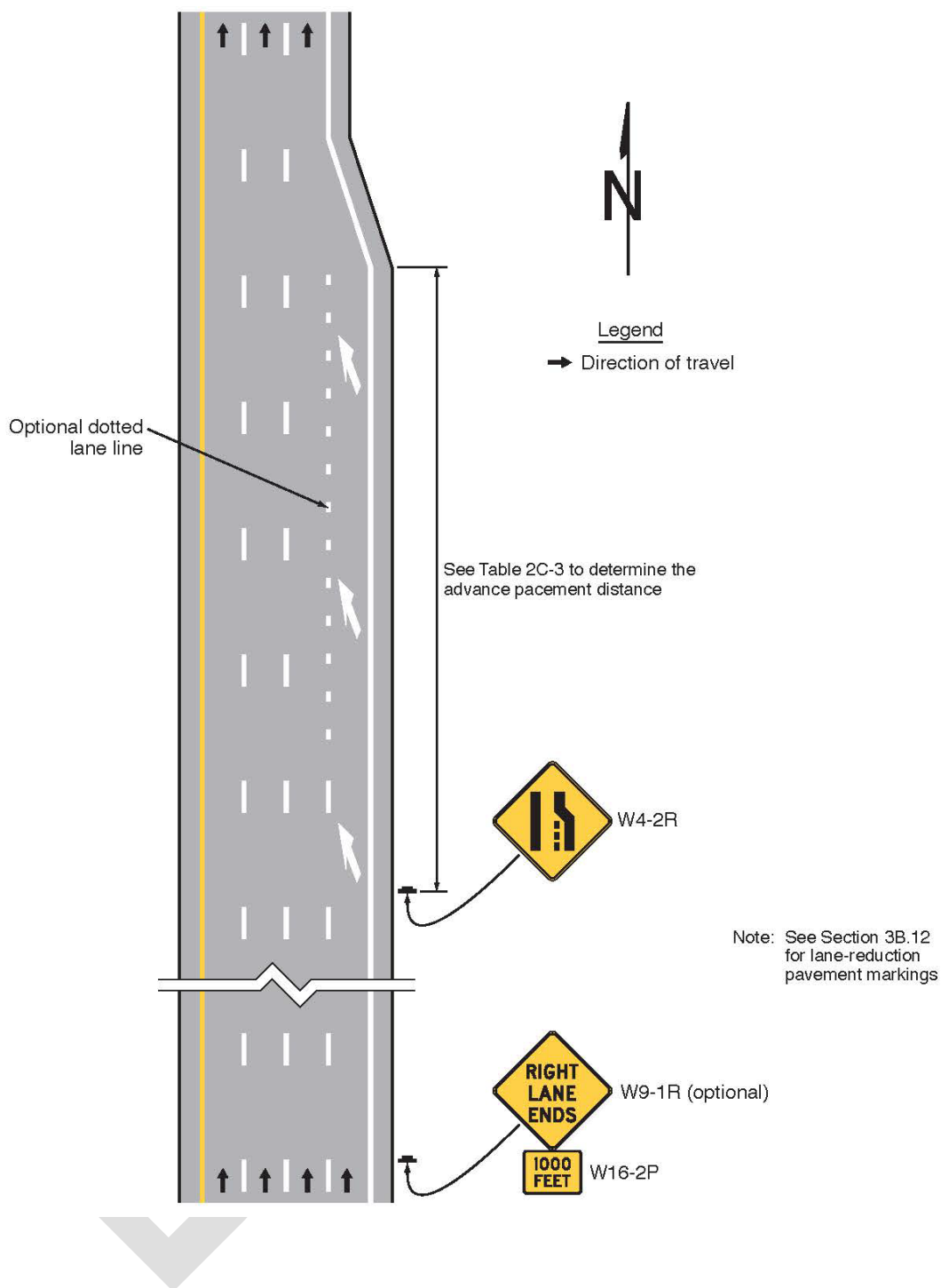
Figure 2C-13. Example Sequences for Lane Ends and Lane Merge Signs (Sheet 1 of 5)
