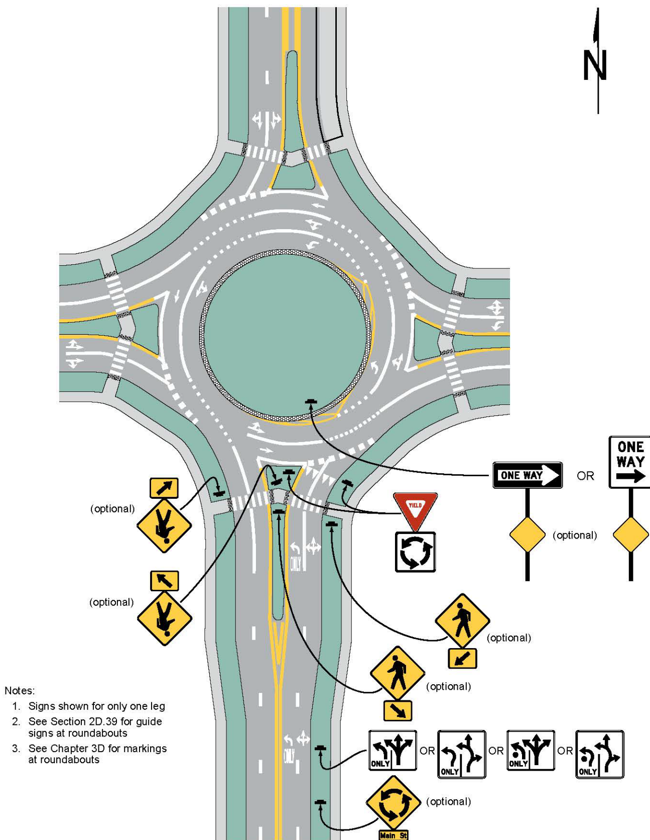
Figure 2B-23. Example of Regulatory and Warning Signs for a Two-Lane Roundabout with Consecutive Double Lefts
