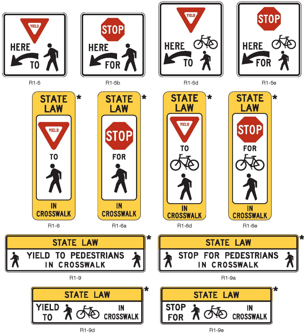
Figure 2B-2. Unsignalized Pedestrian Crosswalk Signs
