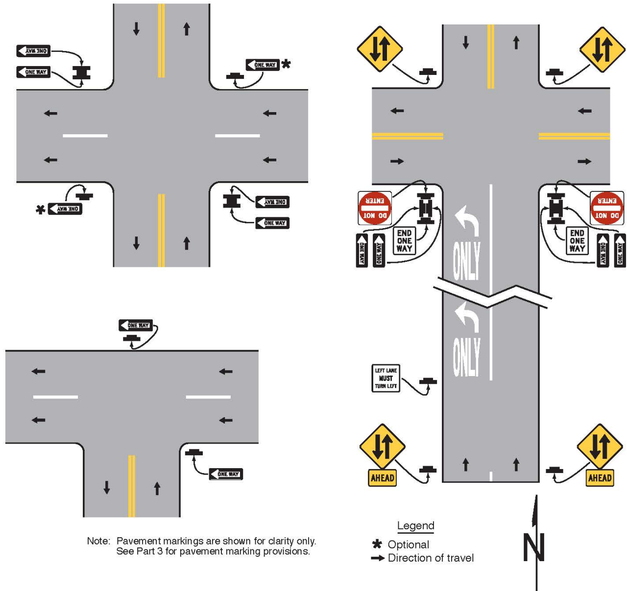
Figure 2B-18. Locations of ONE WAY Signs
