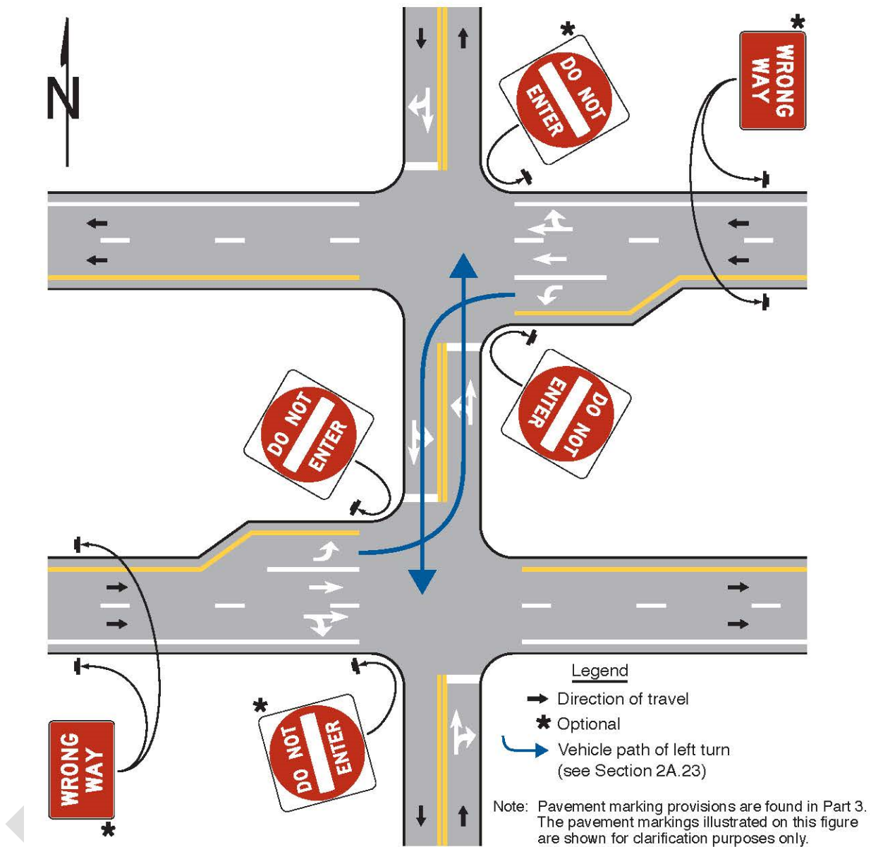
Figure 2B-14. Locations of DO NOT ENTER and WRONG WAY Signing for Divided Highway Crossings that Function as Two Separate Intersections
