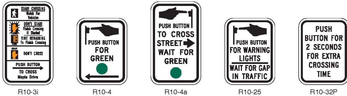
Figure 2B-27. Pedestrian Signs and Plaques (Sheet 2 of 2)
