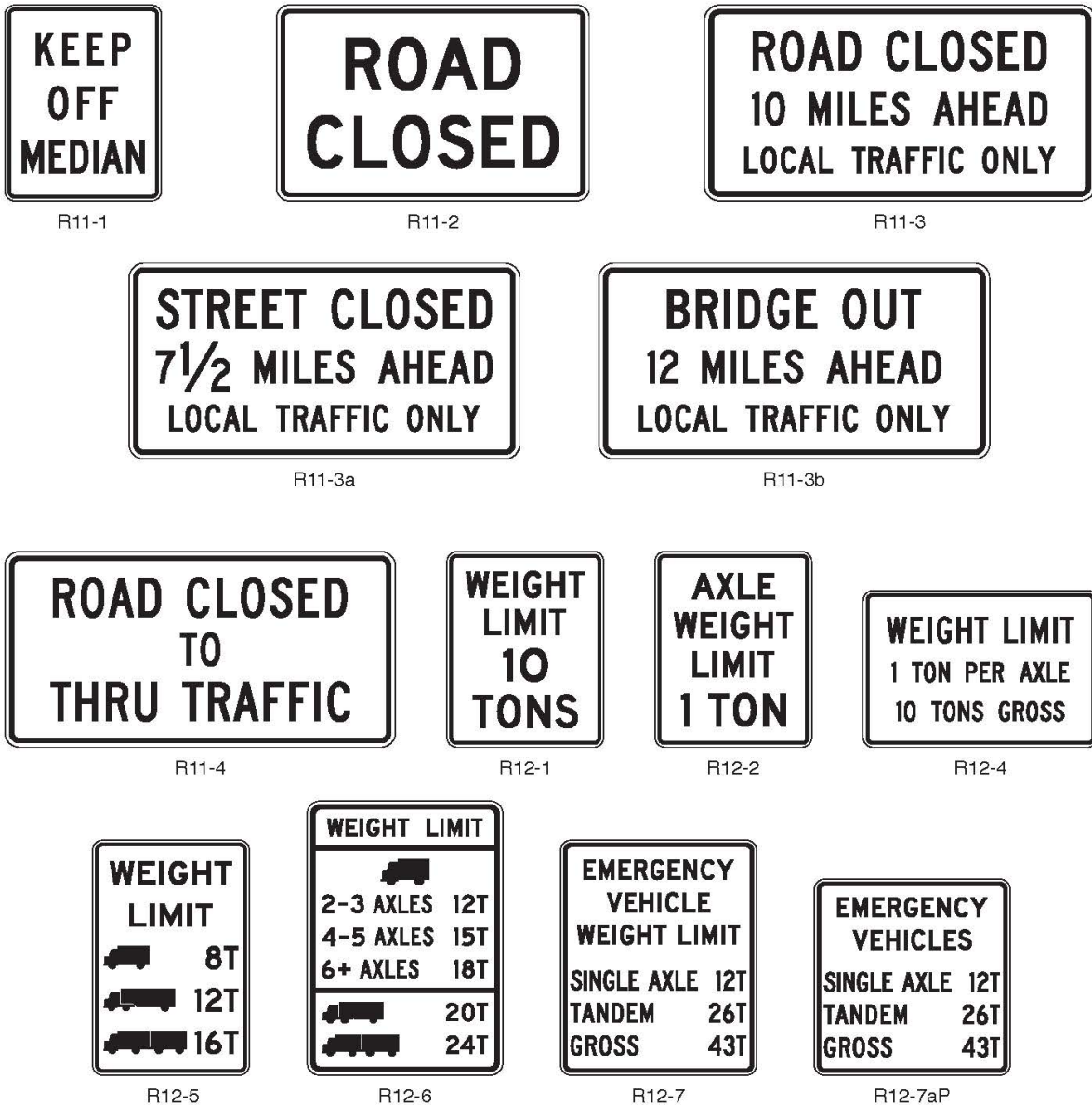
Figure 2B-30. Road Closed and Weight Limit Signs
