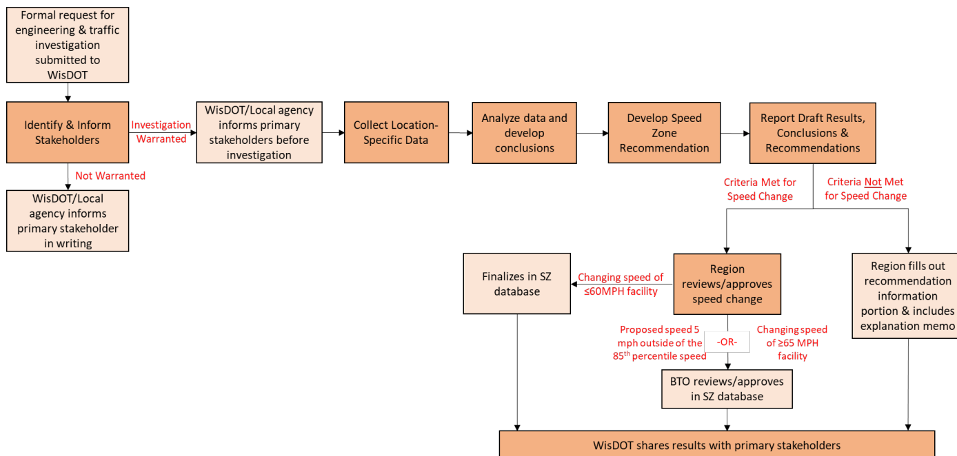
Figure 7.1 Engineering and Traffic Investigation Process
