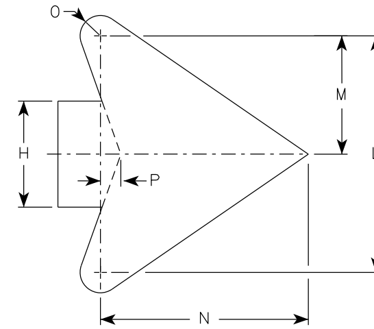
Arrow Detail
