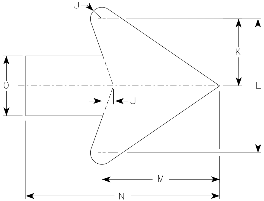
Arrow Detail
