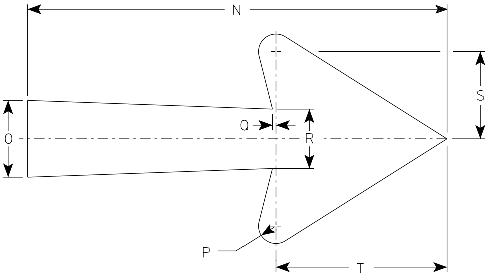
Arrow Detail
