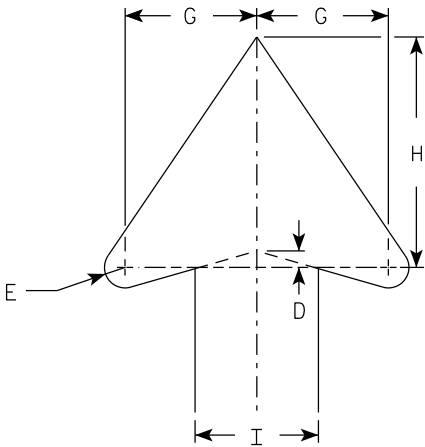
ARROW DETAIL
