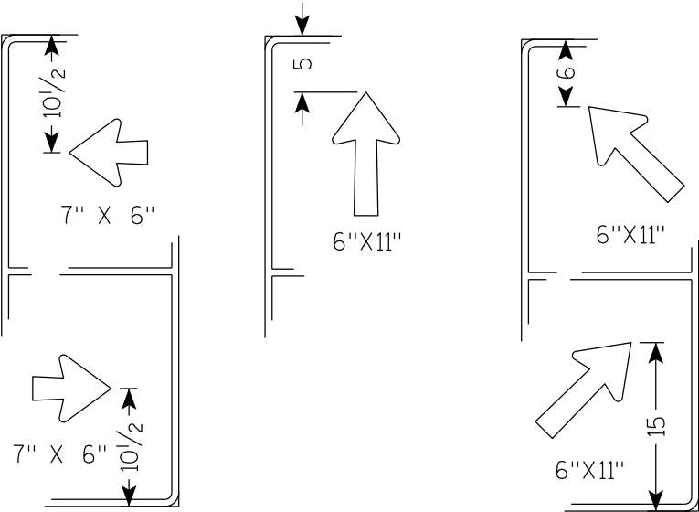
TYPICAL ARROW PLACEMENTS
