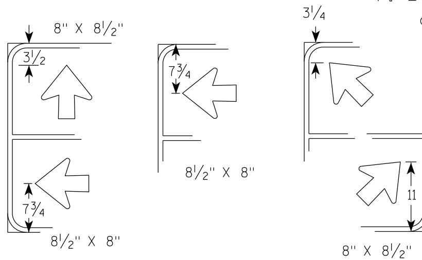
TYPICAL ARROW PLACEMENTS
