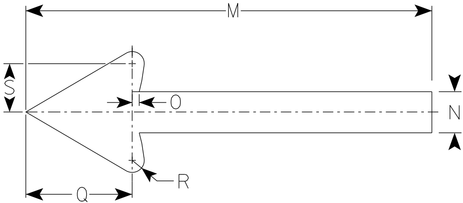
Arrow Detail
