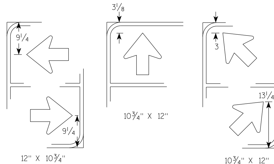
TYPICAL ARROW PLACEMENTS
