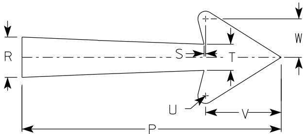
Arrow Detail
