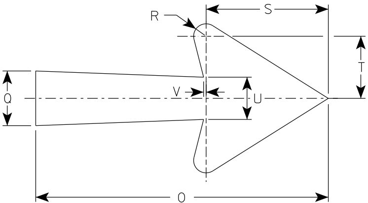
Arrow Detail
