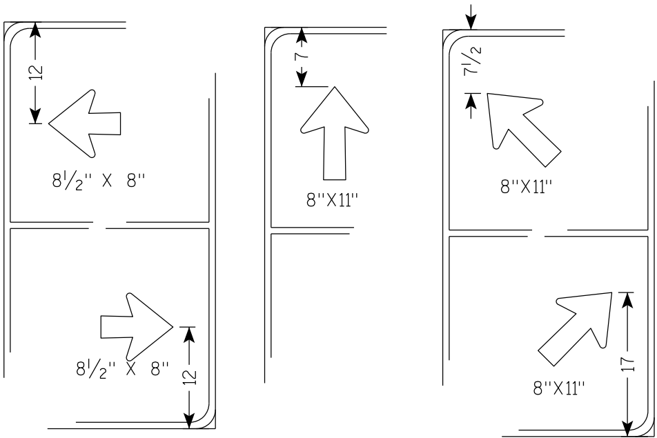
TYPICAL ARROW PLACEMENTS
