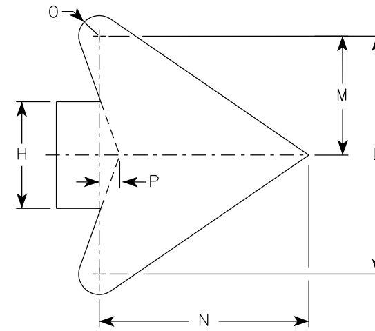
Arrow Detail
