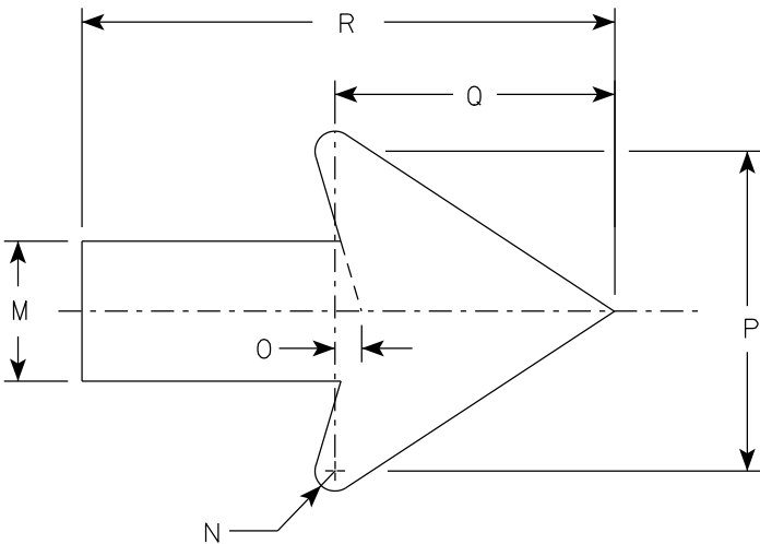
Arrow Detail
