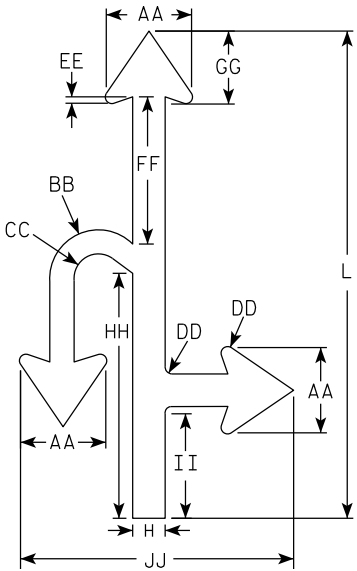
Arrow Detail
