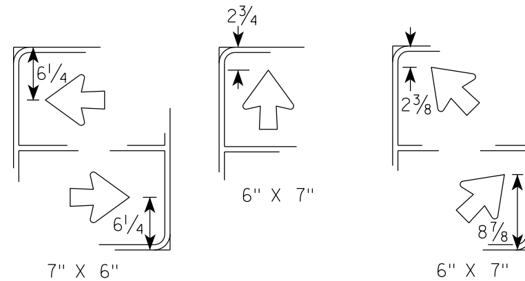
TYPICAL ARROW PLACEMENTS
