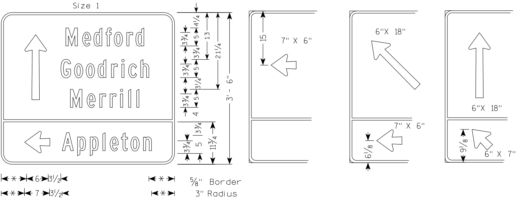
TYPICAL ARROW PLACEMENTS
