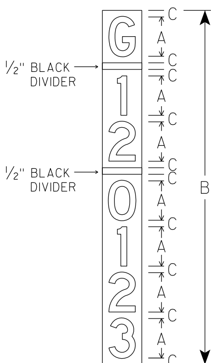
I59-1G RAMP GATE
