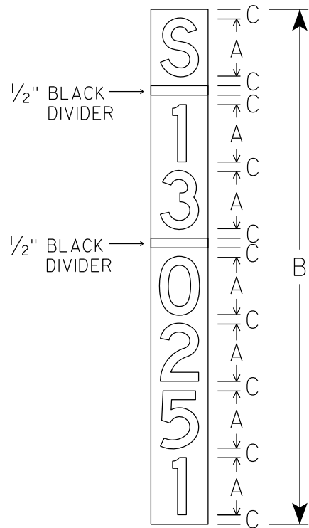
I59-1S SIGN BRIDGE SIGN SUPPORT
