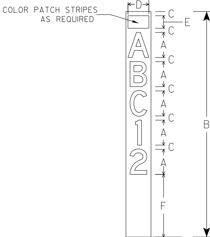
I59-1L LIGHT POLE CIRCUIT/SEQUENCE PLAQUE
