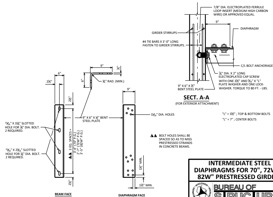
DIAPHRAGM SUPPORT
