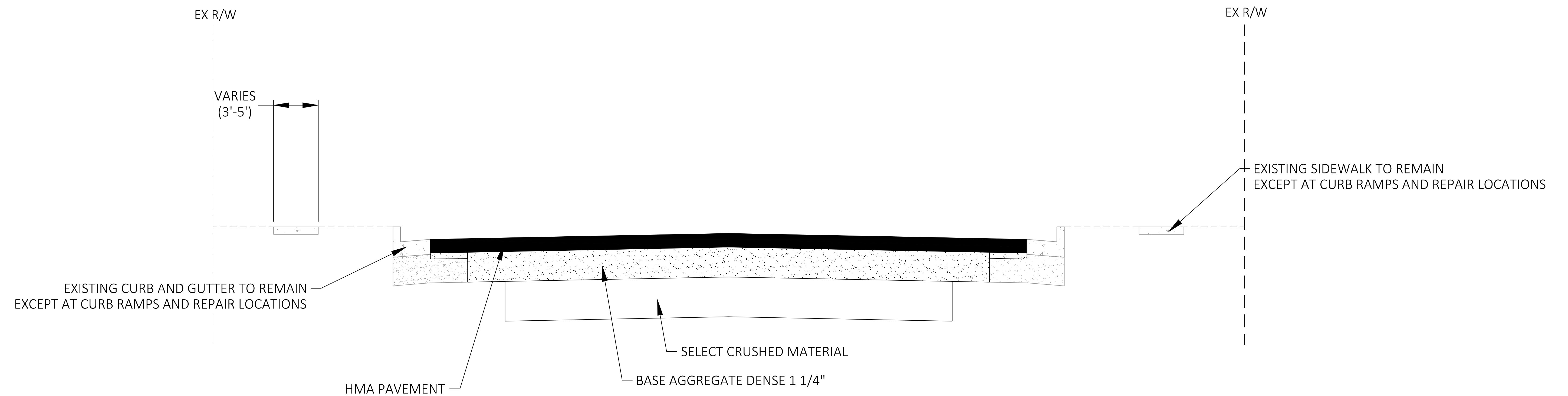
FINISHED TYPICAL SECTION
