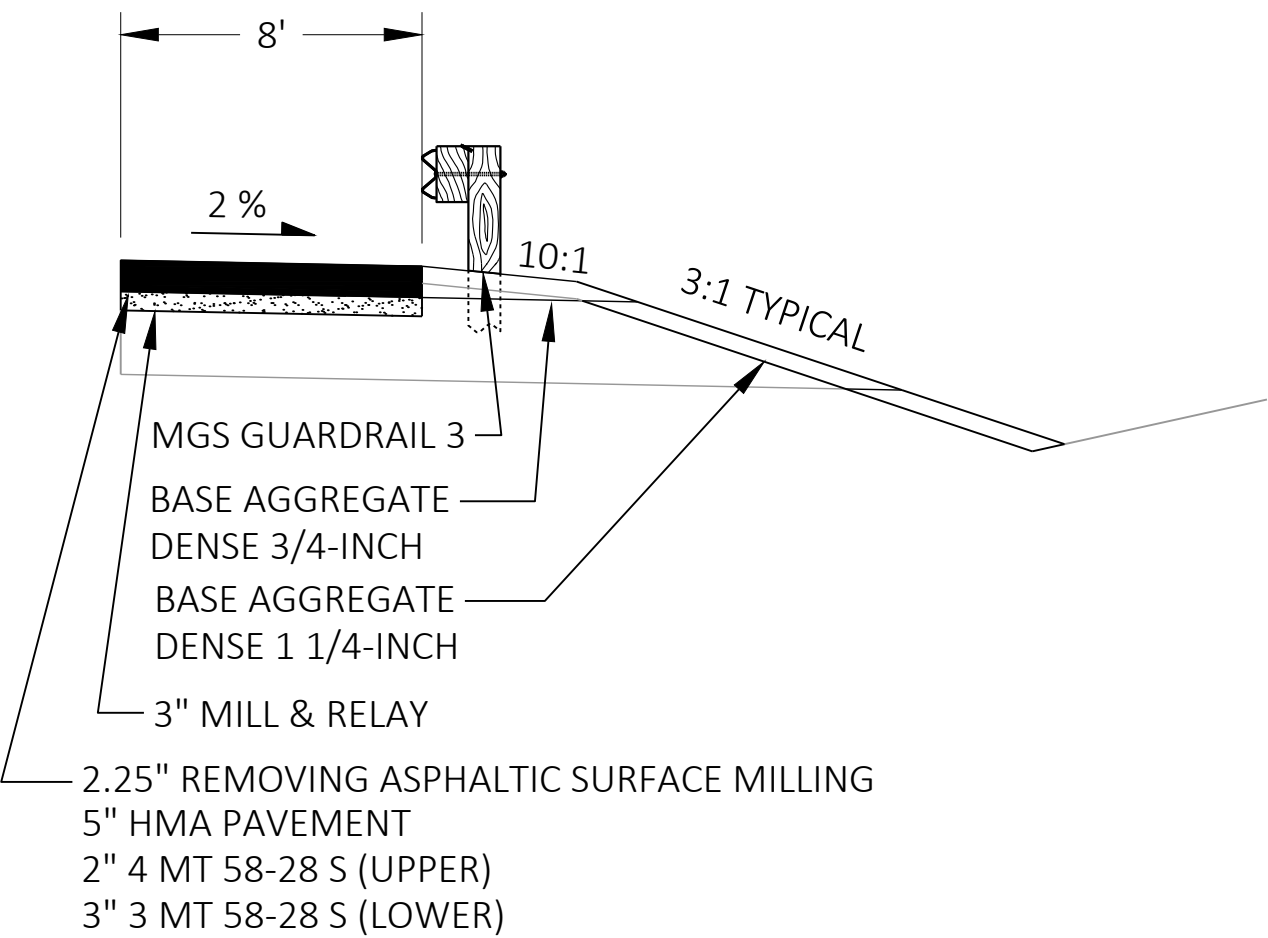
FINISHED BEAMGUARD SECTION STH 35
