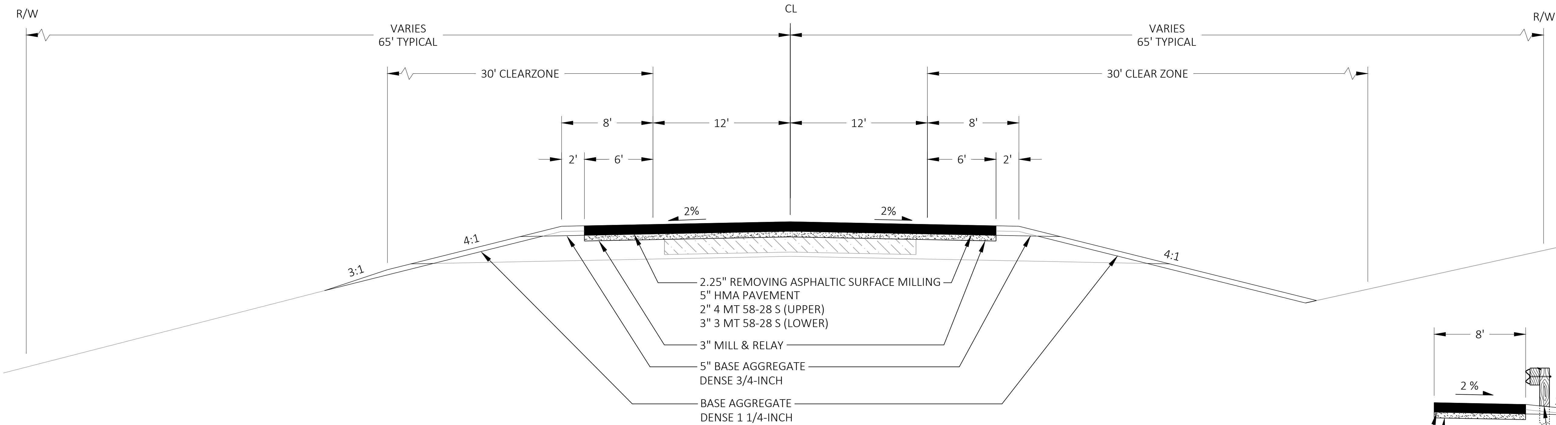
FINISHED TYPICAL SECTION STH 35
