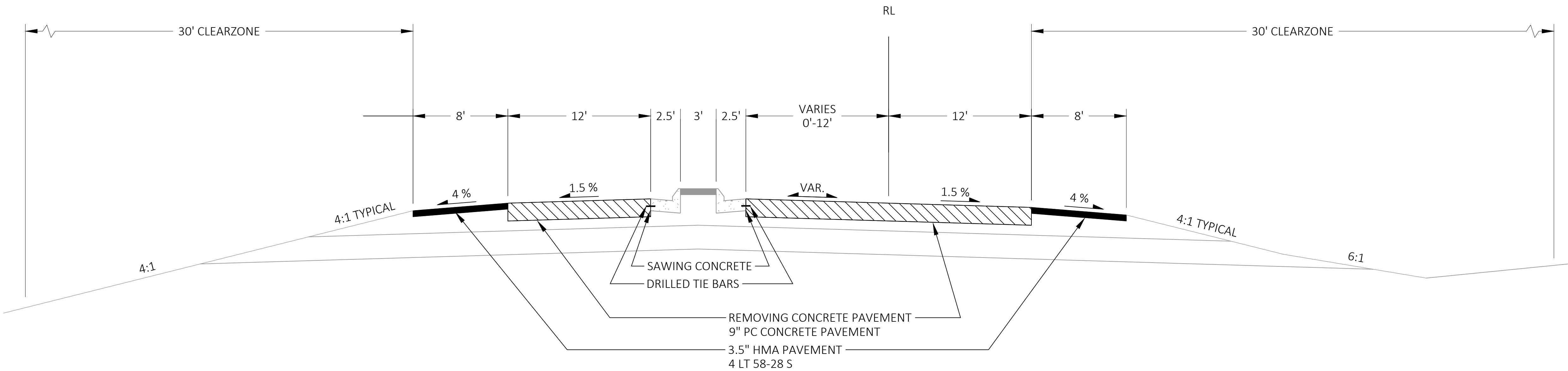
FINISHED TYPICAL SECTION STH 35
