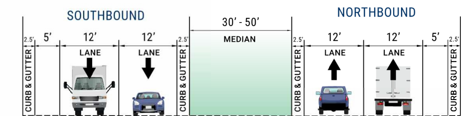
5 Kinsman Boulevard to Pierstorff Street Central Section
