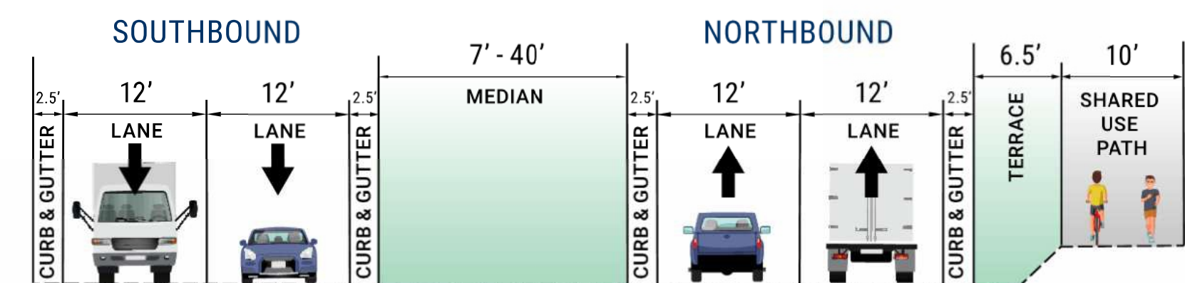
4 Anderson Street to Kinsman Boulevard Central Section
