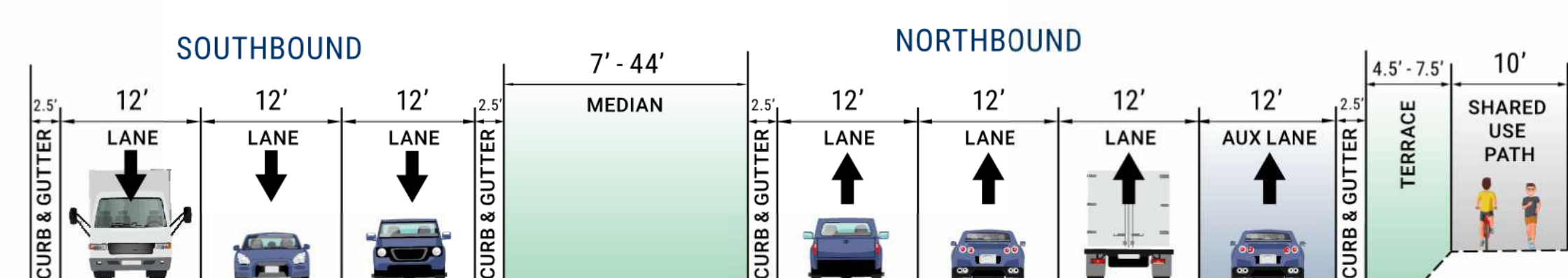
1 South of WIS 30 to Commercial Avenue South Section
