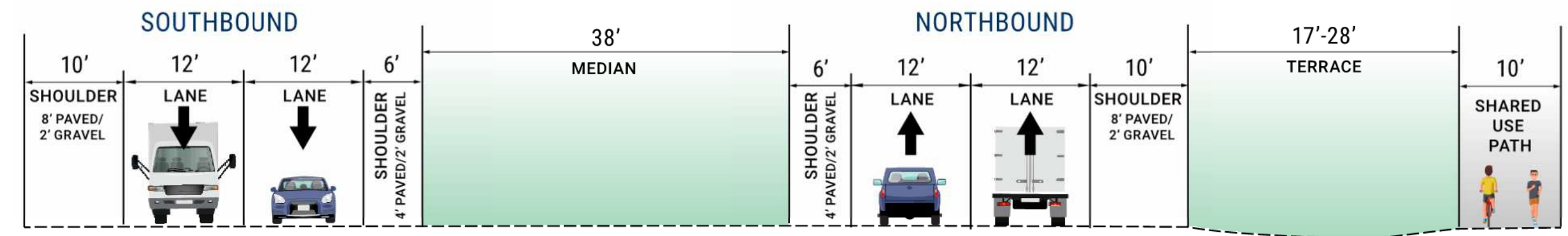
7 Hoepker Road to County CV/Anderson Road North Section
