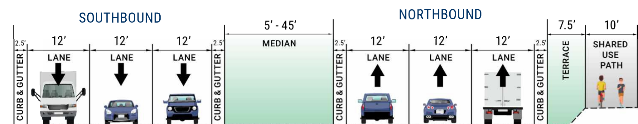
2 Commercial Avenue to US 151 (East Washington Avenue) South Section
