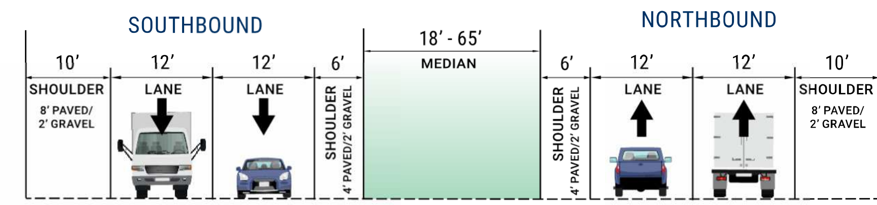
6 Pierstorff Street to Hoepker Road North Section
