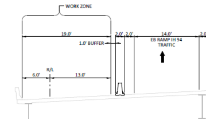
TRAFFIC CONTROL TYPICAL SECTION - STAGE 2 IH 94 EB (SB TO EB RAMP) 8-13-450/455 STA ____ TO STA ____
