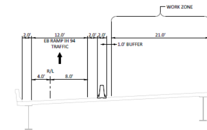
TRAFFIC CONTROL TYPICAL SECTION - STAGE 1 IH 94 EB (SB TO EB RAMP) 8-13-450/455 STA ____ TO STA ____
