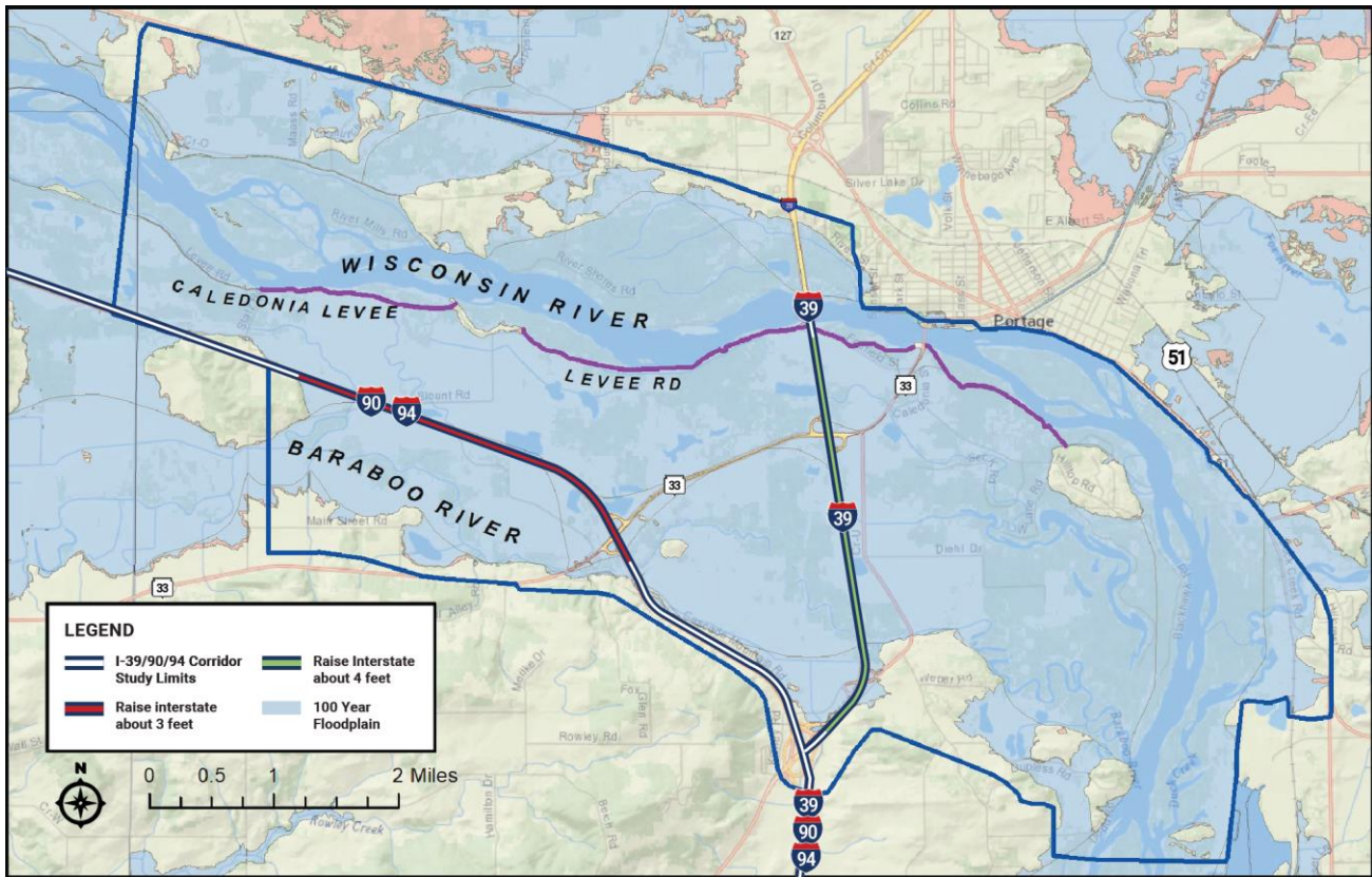
Figure 3-38: Location of Increased Interstate Elevation
