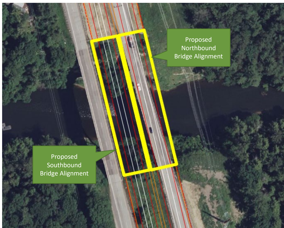
Figure 3. Proposed Mirror Bridge Alignment
