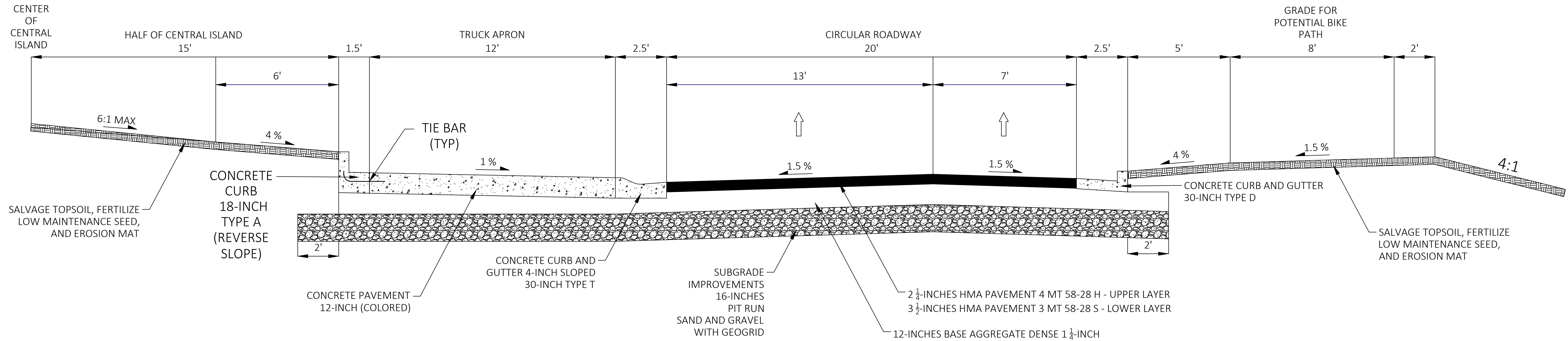
PROPOSED TYPICAL HALF-SECTION STH 11 AND COUNTY F ROUNDABOUT
