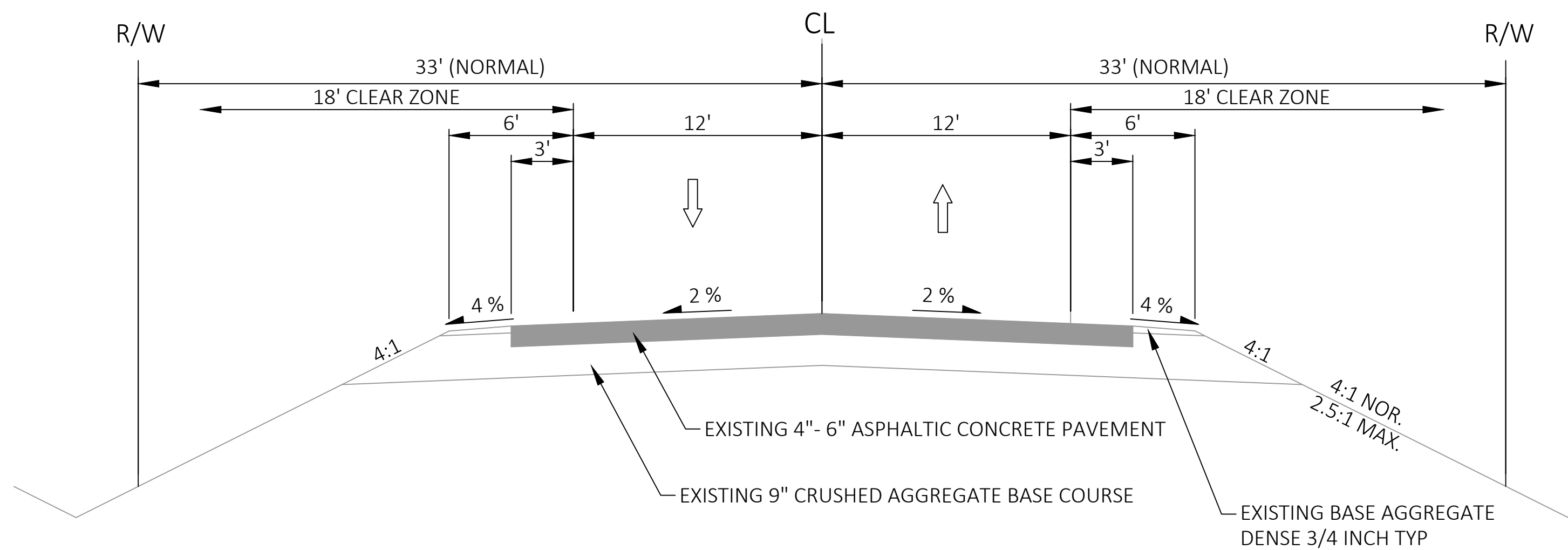
EXISTING TYPICAL SECTION - STH 11 (LIMITS FOR ROUNDABOUT, 3841-05-76)
