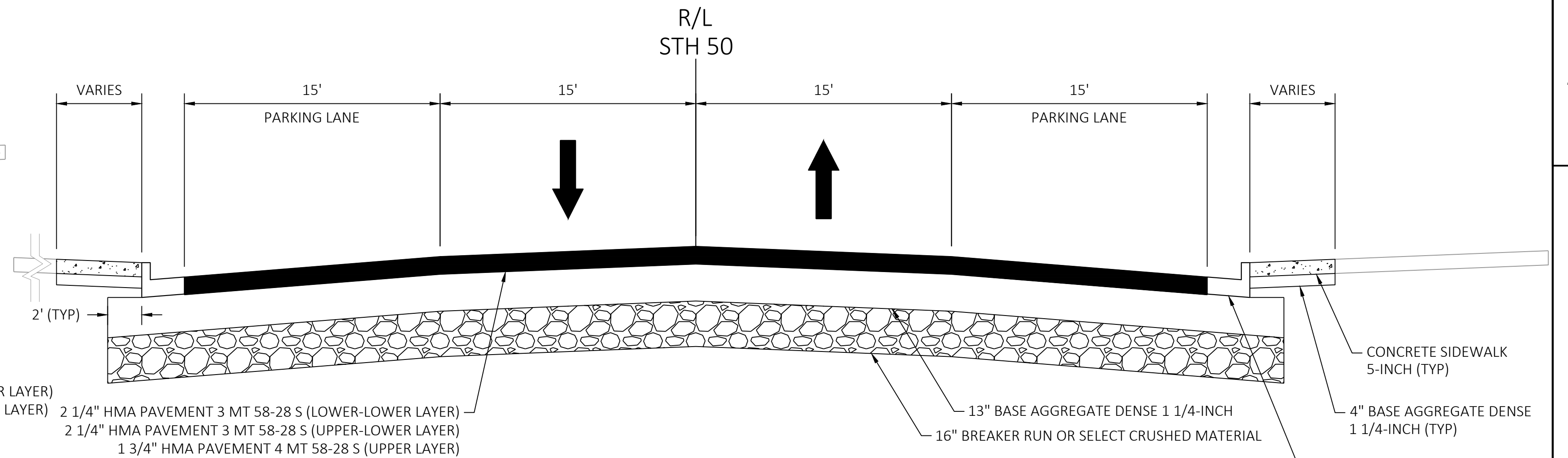
FINISHED TYPICAL SECTION SEGMENT 2
