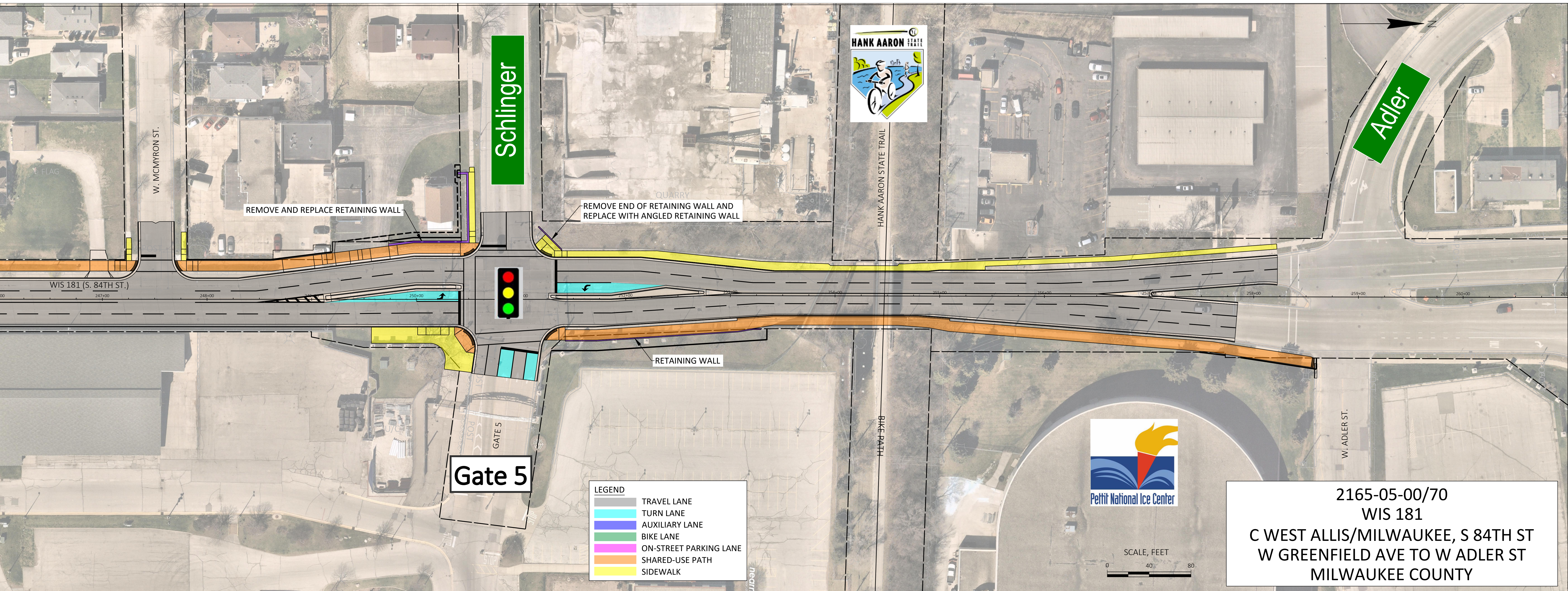
WIS 181 SHARED-USE PATH ALTERNATIVE (W. GREENFIELD AVENUE TO W. ADLER STREET)
