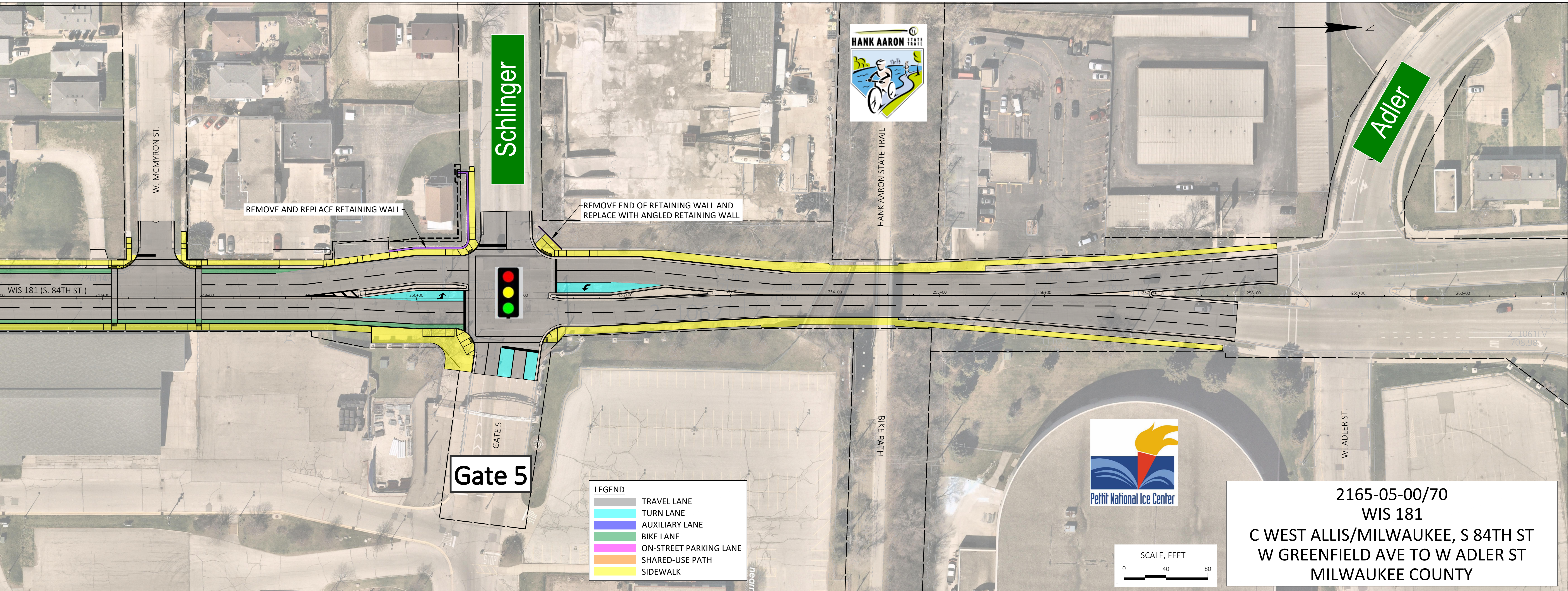
WIS 181 ON-STREET BICYCLE ACCOMMODATIONS ALTERNATIVE (W. GREENFIELD AVENUE TO W. ADLER STREET)
