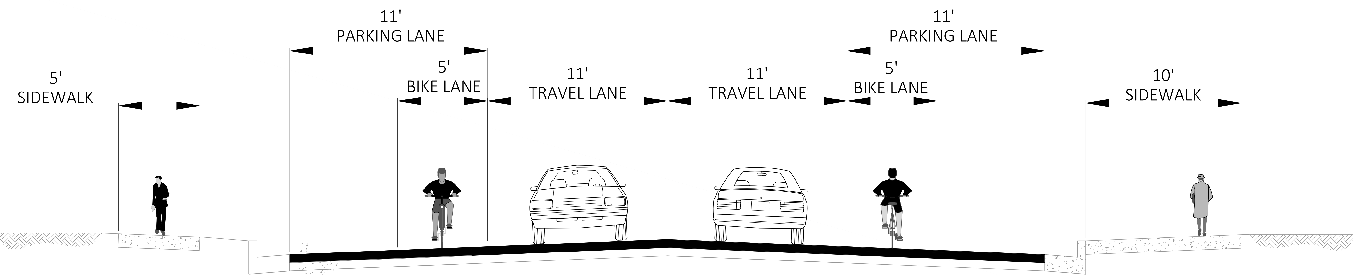
PROPOSED TYPICAL SECTION - WIS 175 FROM SLINGER RD/SCENIC AVE TO KETTLE MORaine DR
