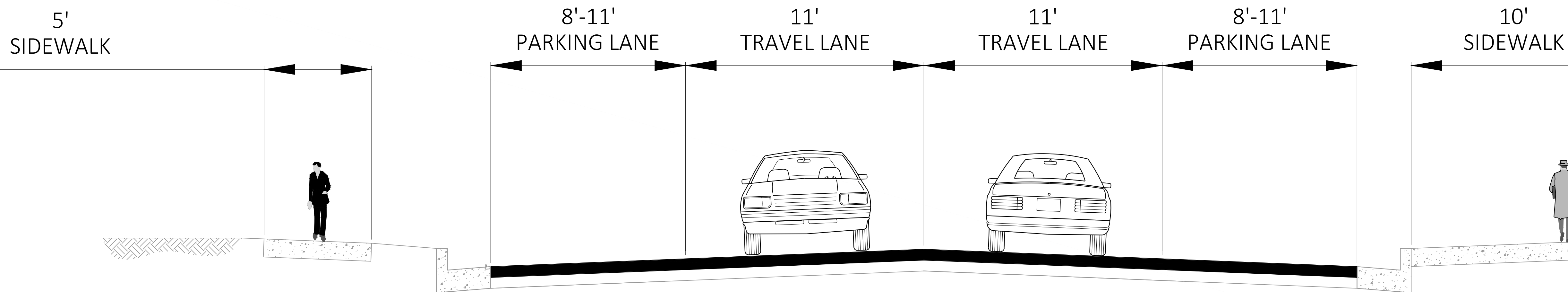
PROPOSED TYPICAL SECTION - WIS 175 FROM KETTLE MORaine DR TO N MAPLE AVE
