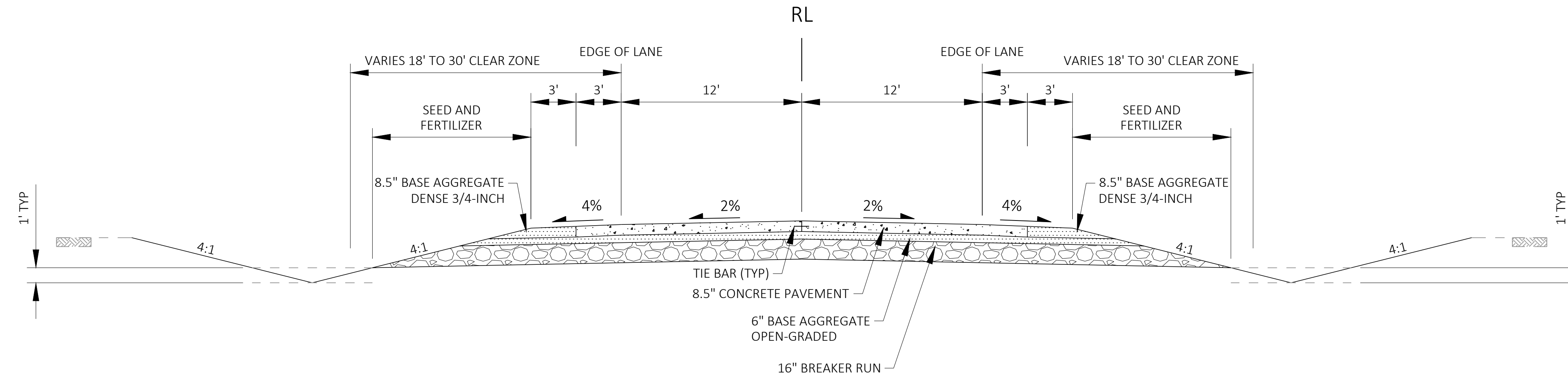
FINISHED TYPICAL SECTION - US 14 KNOLL ROAD TO ILLINOIS STATE LINE
