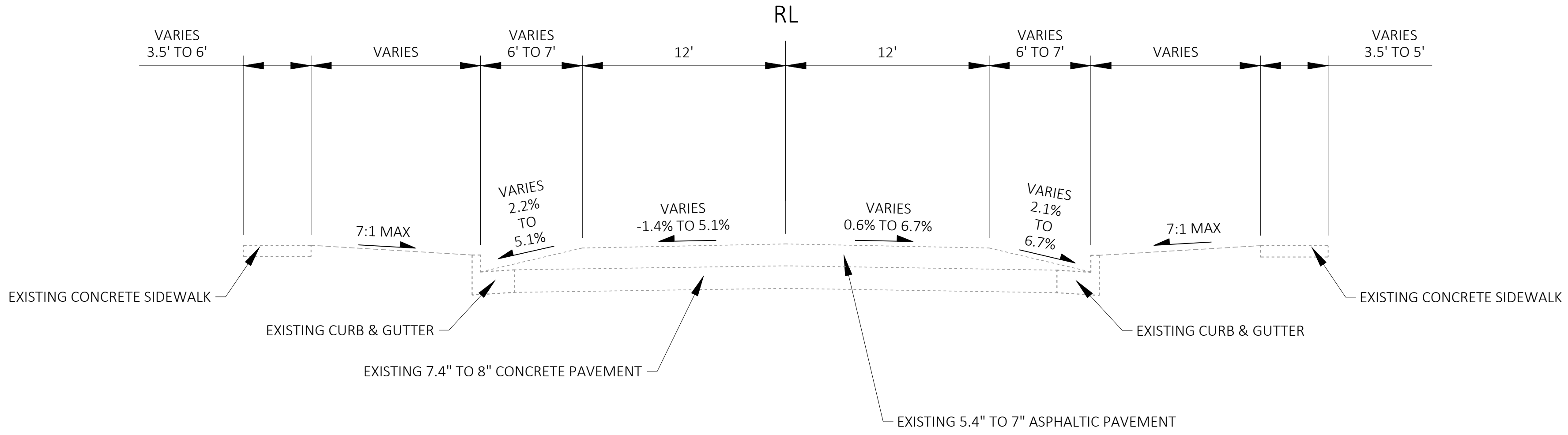
FINISHED TYPICAL SECTION - US 14 NORTH VILLAGE LIMITS TO VILLAGE SQUARE MAPLE STREET TO FAIRVIEW DRIVE
