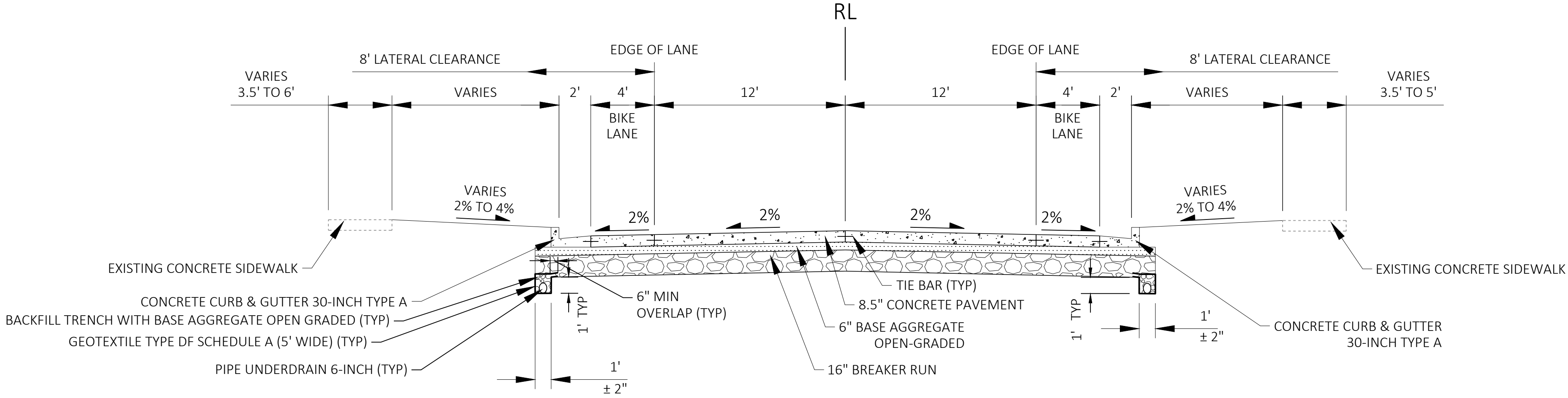
FINISHED TYPICAL SECTION - US 14 NORTH VILLAGE LIMITS TO VILLAGE SQUARE MAPLE STREET TO FAIRVIEW DRIVE
