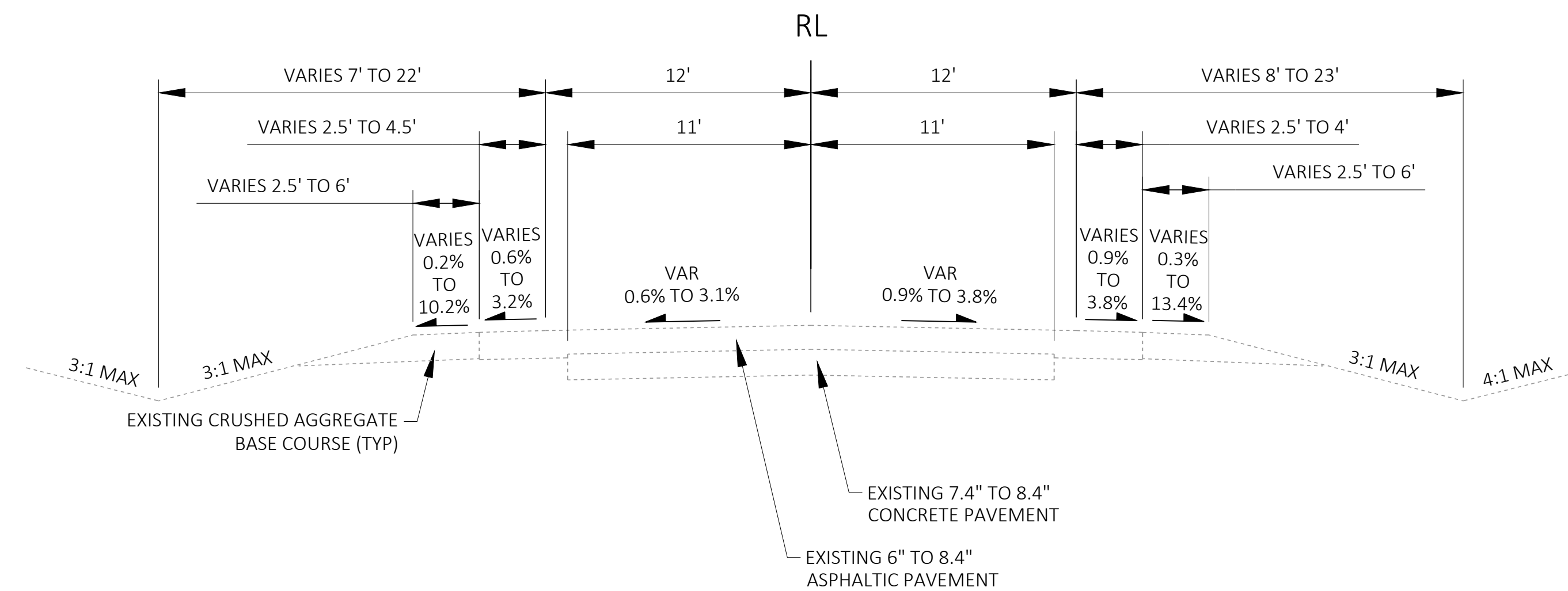
EXISTING TYPICAL SECTION - US 14 KNOLL ROAD TO ILLINOIS STATE LINE
