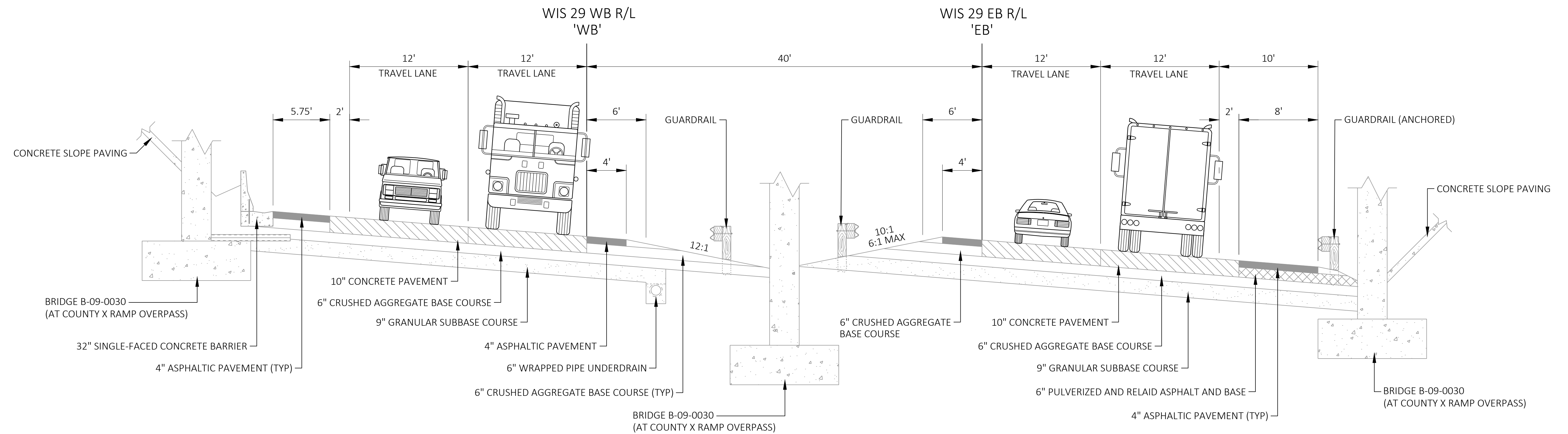
EXISTING TYPICAL SECTION - WIS 29 AT COUNTY X RAMP OVERPASS
