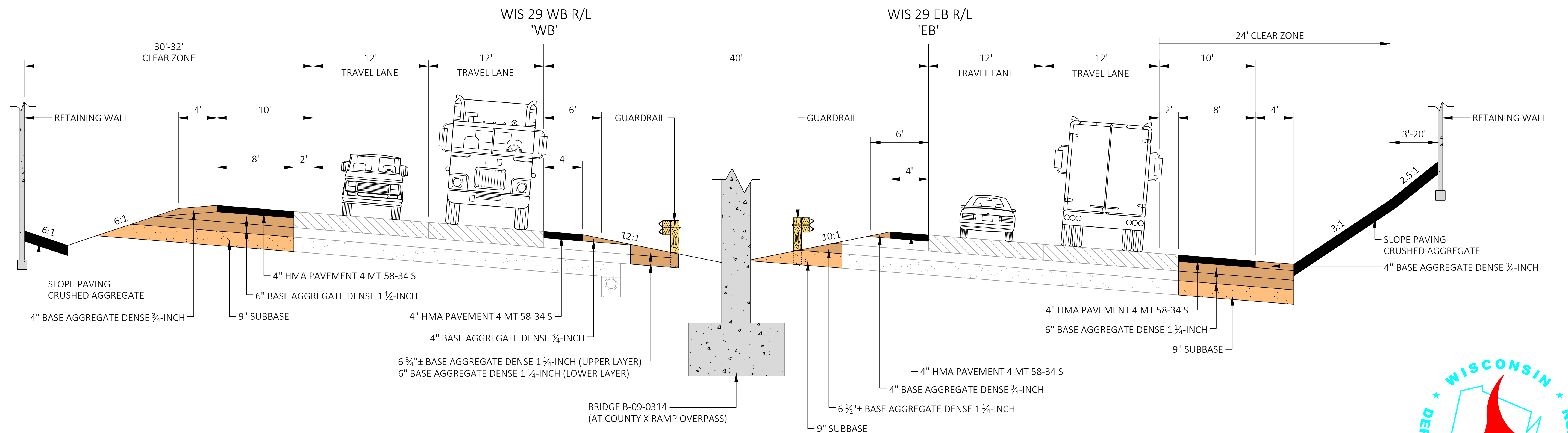
PROPOSED TYPICAL SECTION - WIS 29 AT COUNTY X RAMP OVERPASS
