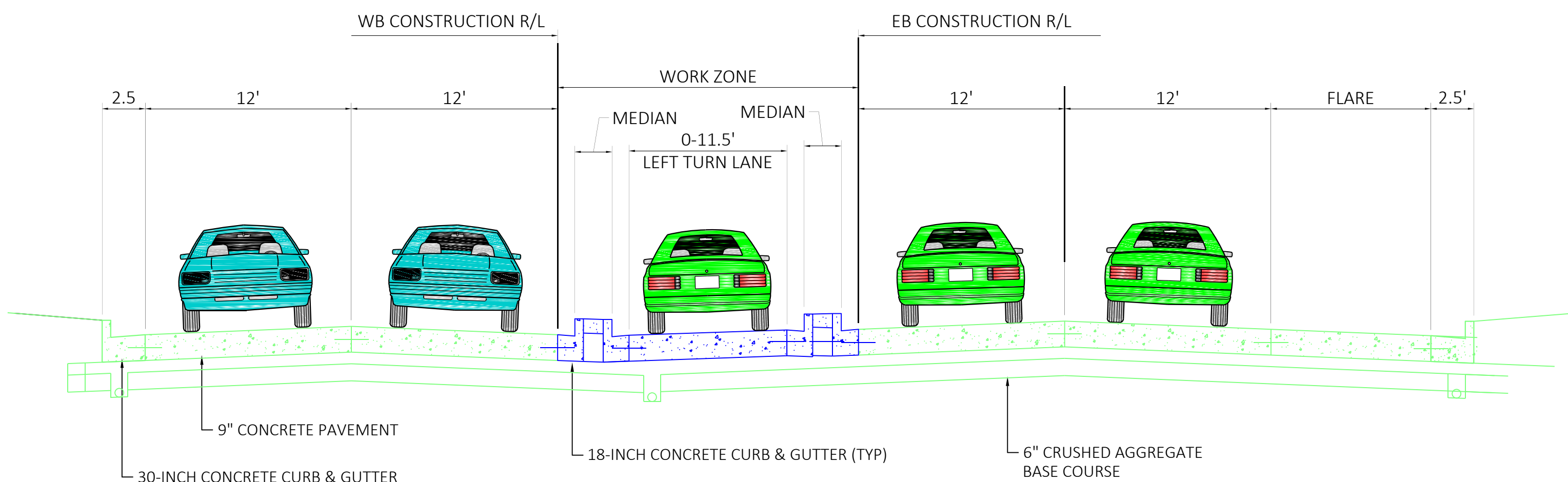
FINISHED TYPICAL CROSS SECTION STH 32 WITH WB TURNING LANES
