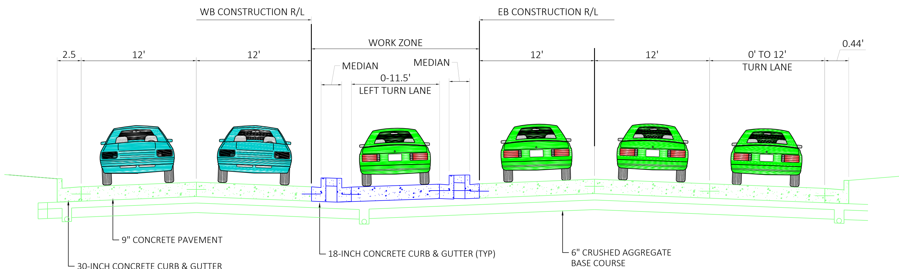
FINISHED TYPICAL CROSS SECTION STH 32 WITH EB TURNING LANES
