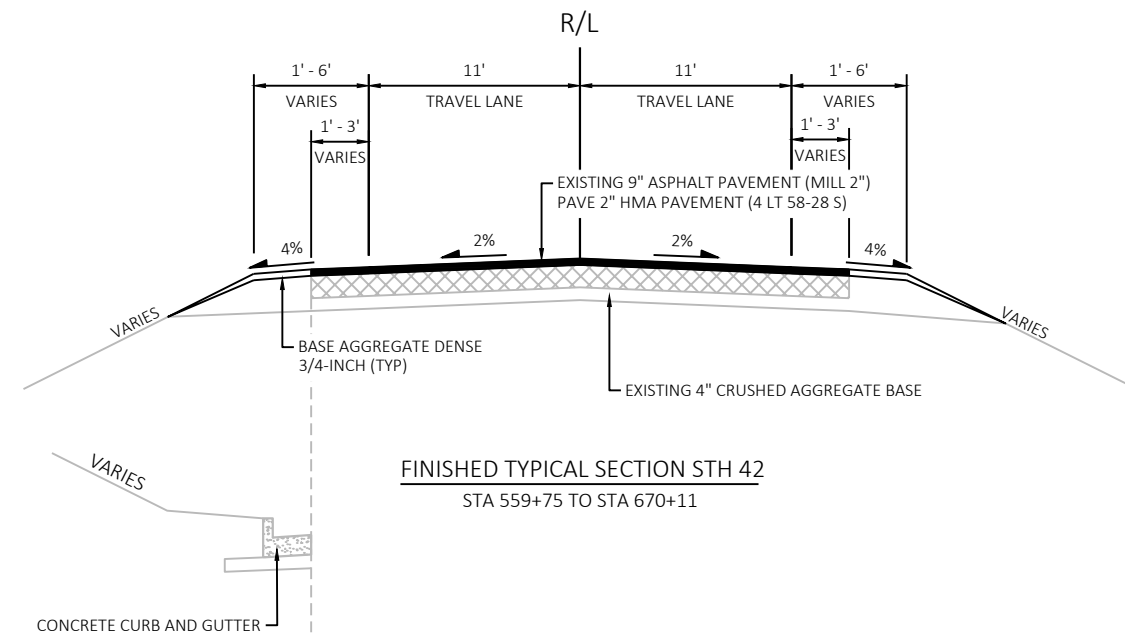
TYPICAL HALF SECTION SHOULDER CURB STA 572+28 TO STA 577+37
