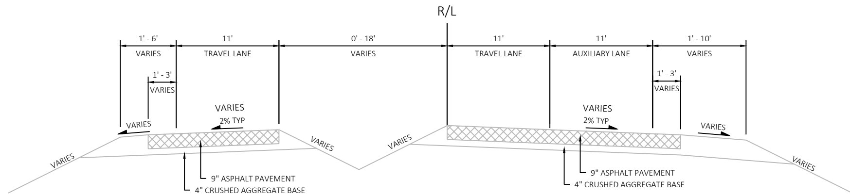
EXISTING TYPICAL SECTION STH 42 STA 670+11 TO STA 676+20
