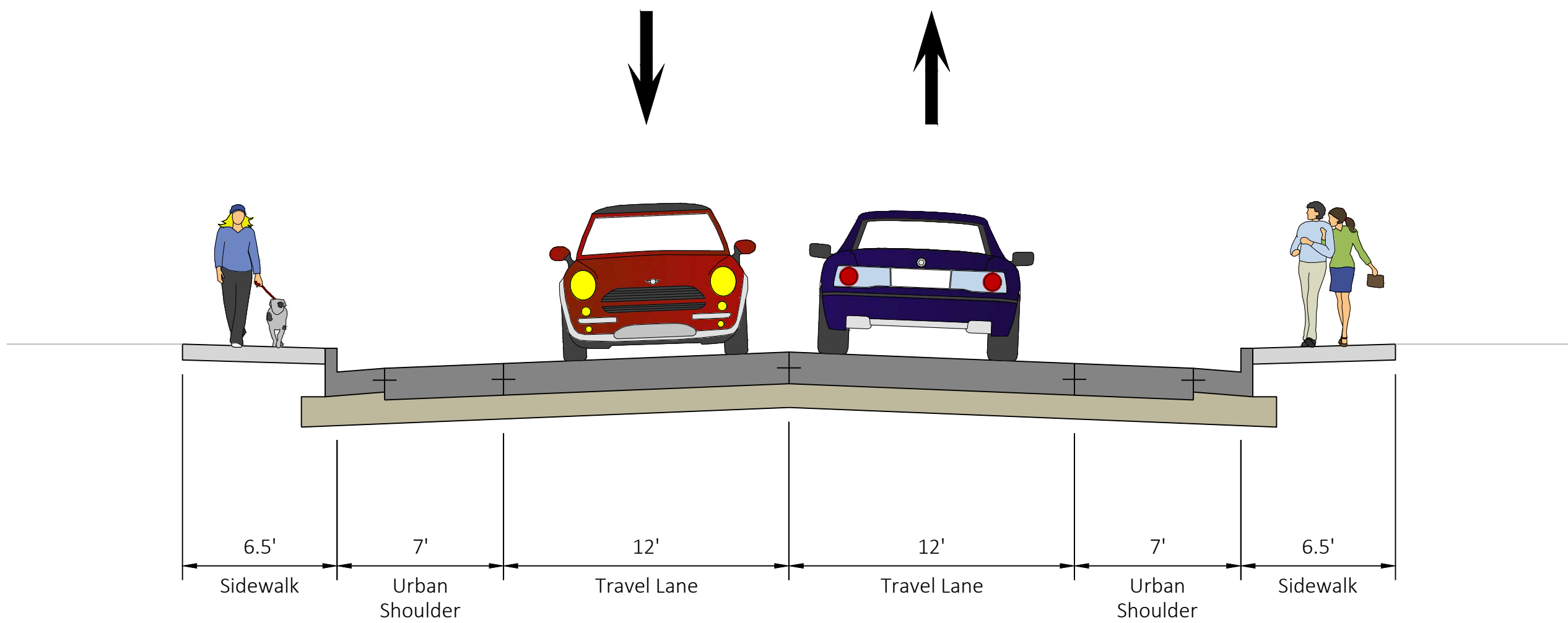
Proposed Typical Section
