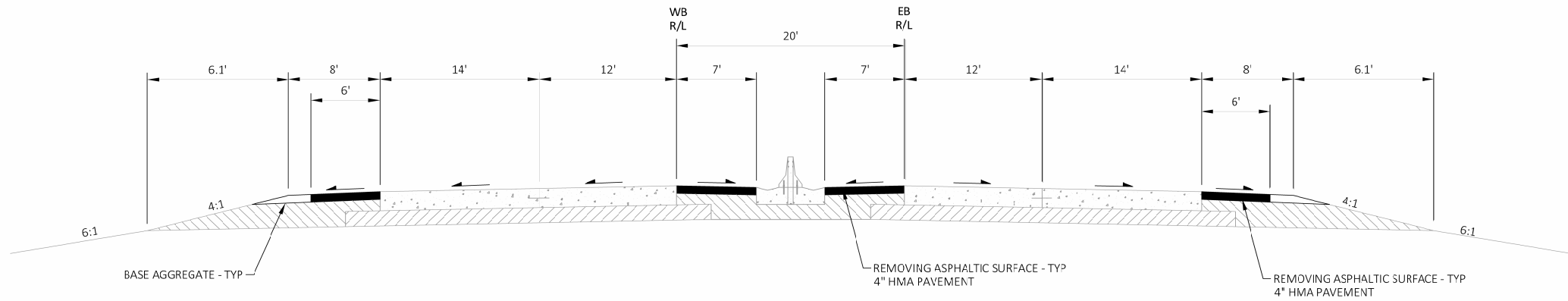
FINISHED TYPICAL SECTION
