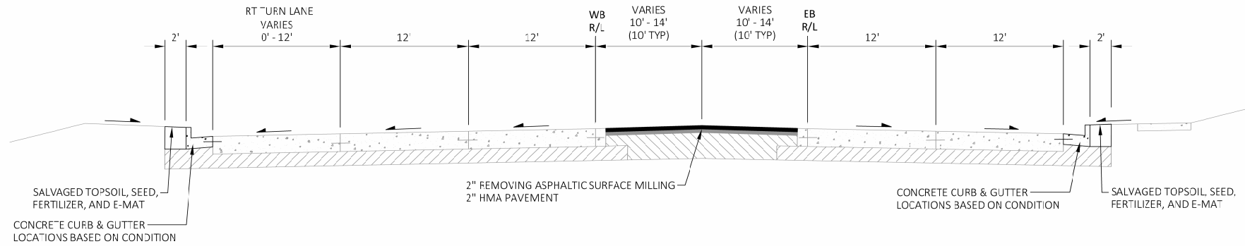
FINISHED TYPICAL SECTION
