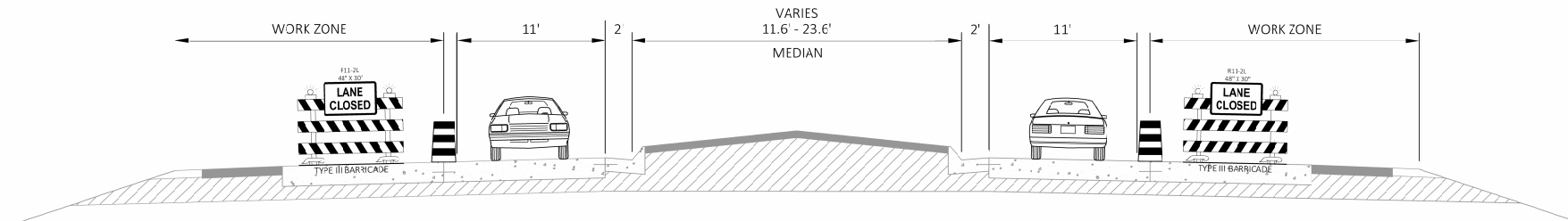
TRAFFIC CONTROL TYPICAL SECTION CTH J - OUTSIDE LANE CLOSURE
