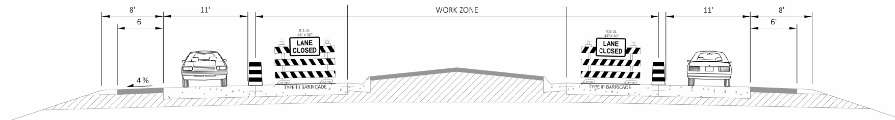
TRAFFIC CONTROL TYPICAL SECTION CTH J - INSIDE LANE CLOSURE
