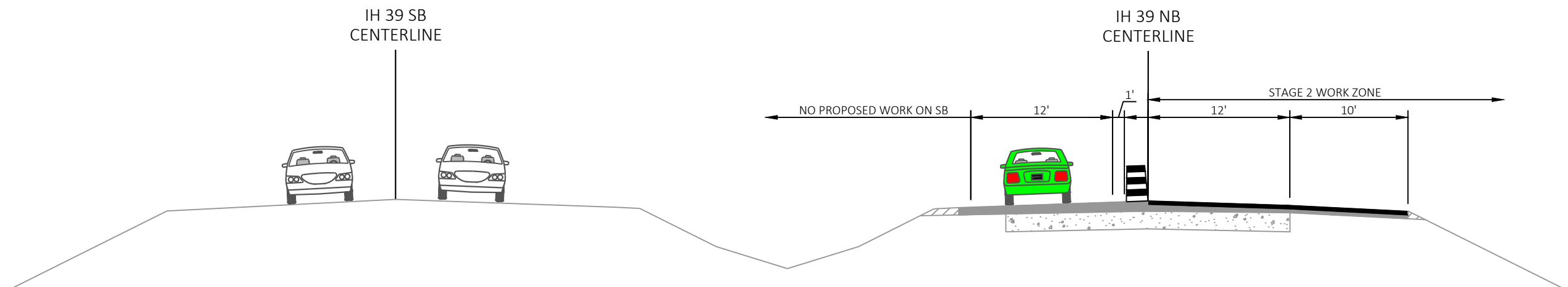
STAGE 2 LOOKING NORTH MILL AND OVERLAY OUTSIDE TRAVEL LANE AND SHOULDER
