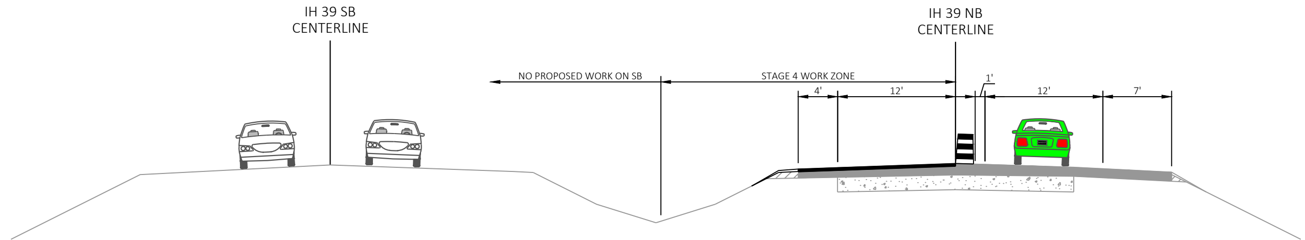
STAGE 4 LOOKING NORTH PAVE INSIDE TRAVEL LANE AND SHOULDER
