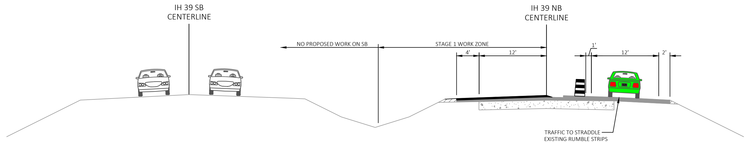
STAGE 1 LOOKING NORTH MILL AND OVERLAY INSIDE TRAVEL LANE AND SHOULDER
