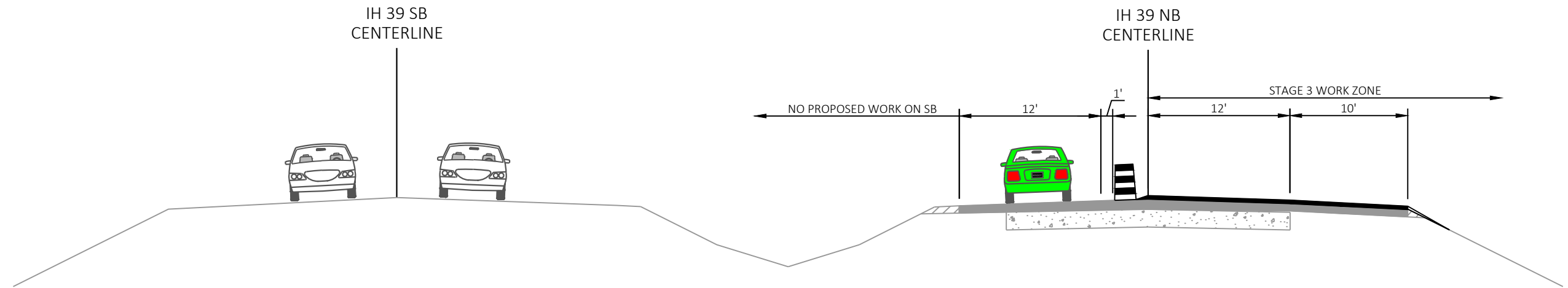
STAGE 3 LOOKING NORTH PAVE OUTSIDE TRAVEL LANE AND SHOULDER
