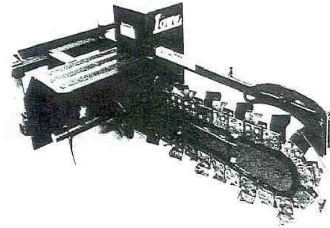
Class 9178 Earth Saw or Trenching attachment
