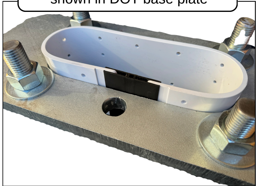
Oval Rodent Barrier shown in DOT base plate
