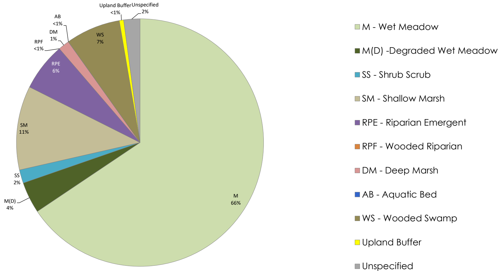
Figure 1. 2022 Available Wetland Mitigation Credits by Wetland Type
