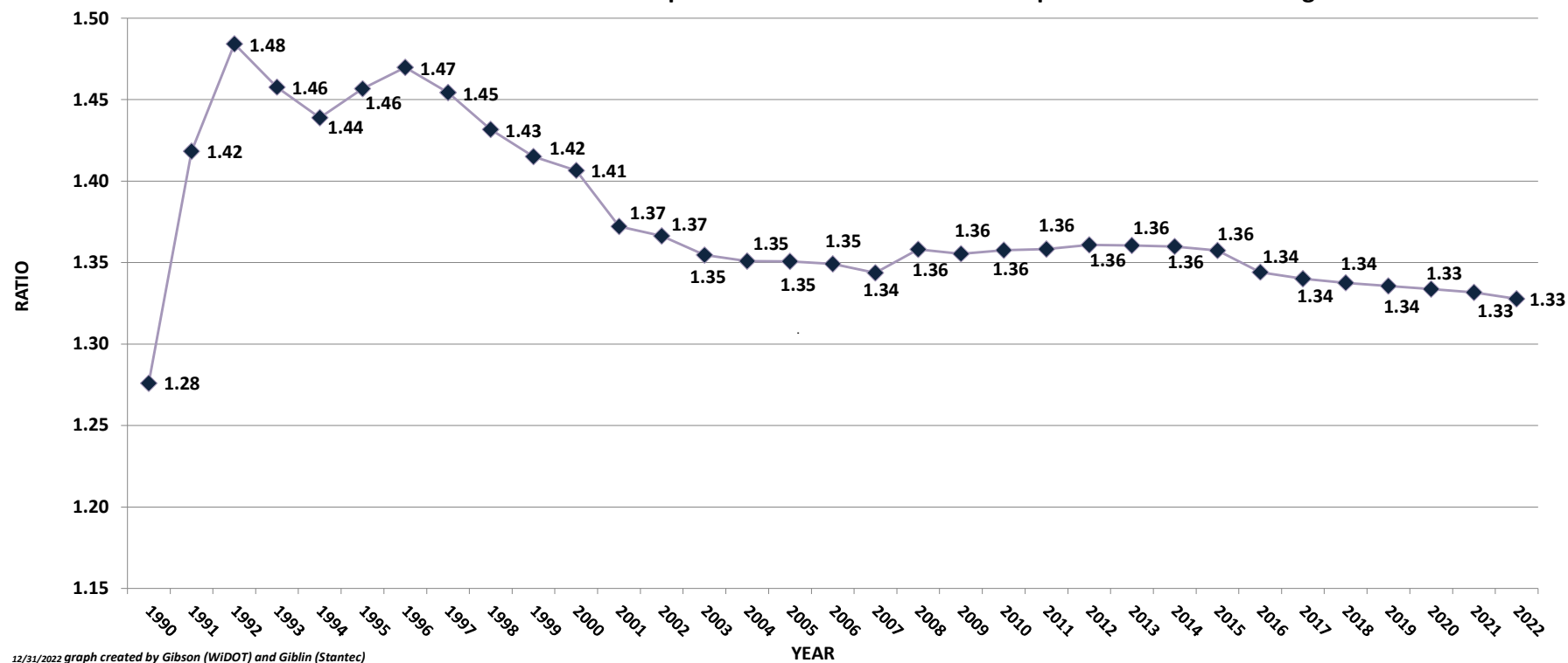
Ratio of WisDOT Cumulative Acres Compensated to Cumulative Acres Impacted from 1990 through 2022
