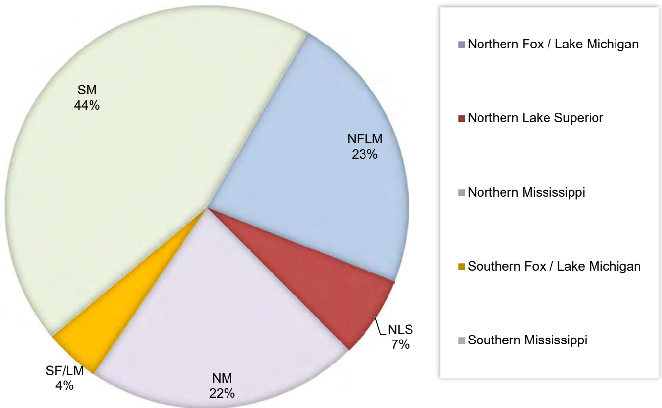
Figure 1. 2022 WisDOT Wetland Loss by Wetland Bank Region
