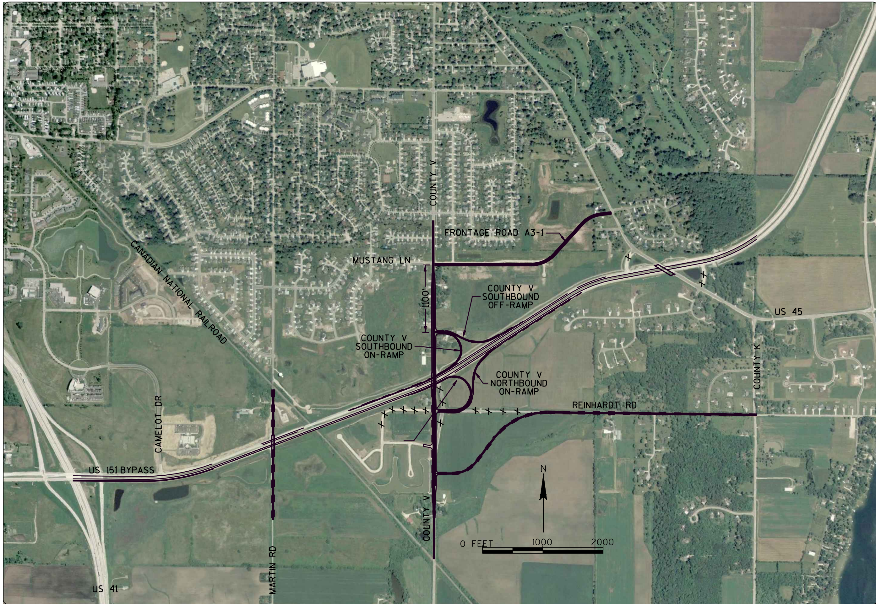
US 151 MIDDLE ALTERNATIVE FRONTAGE ROAD OPTION A3-1 5-1-08
