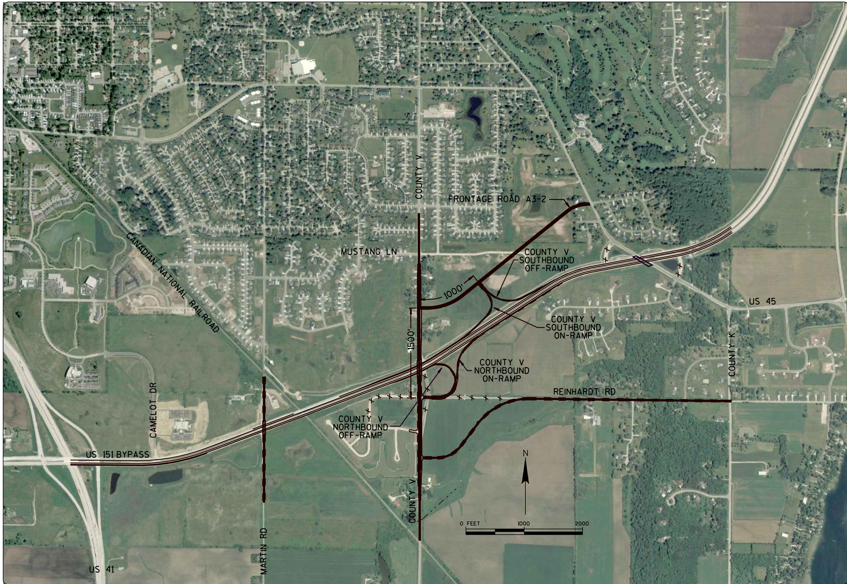
US 151 MIDDLE ALTERNATIVE FRONTAGE ROAD OPTION A3-2 5-21-08
