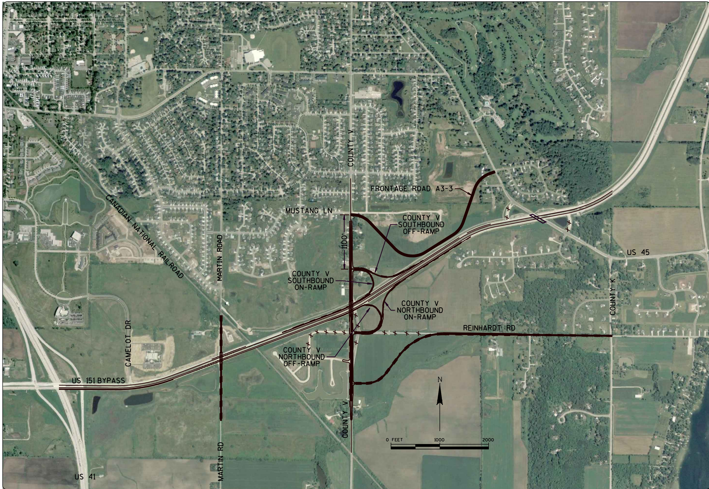
US 151 MIDDLE ALTERNATIVE FRONTAGE ROAD OPTION A3-3 5-1-08
