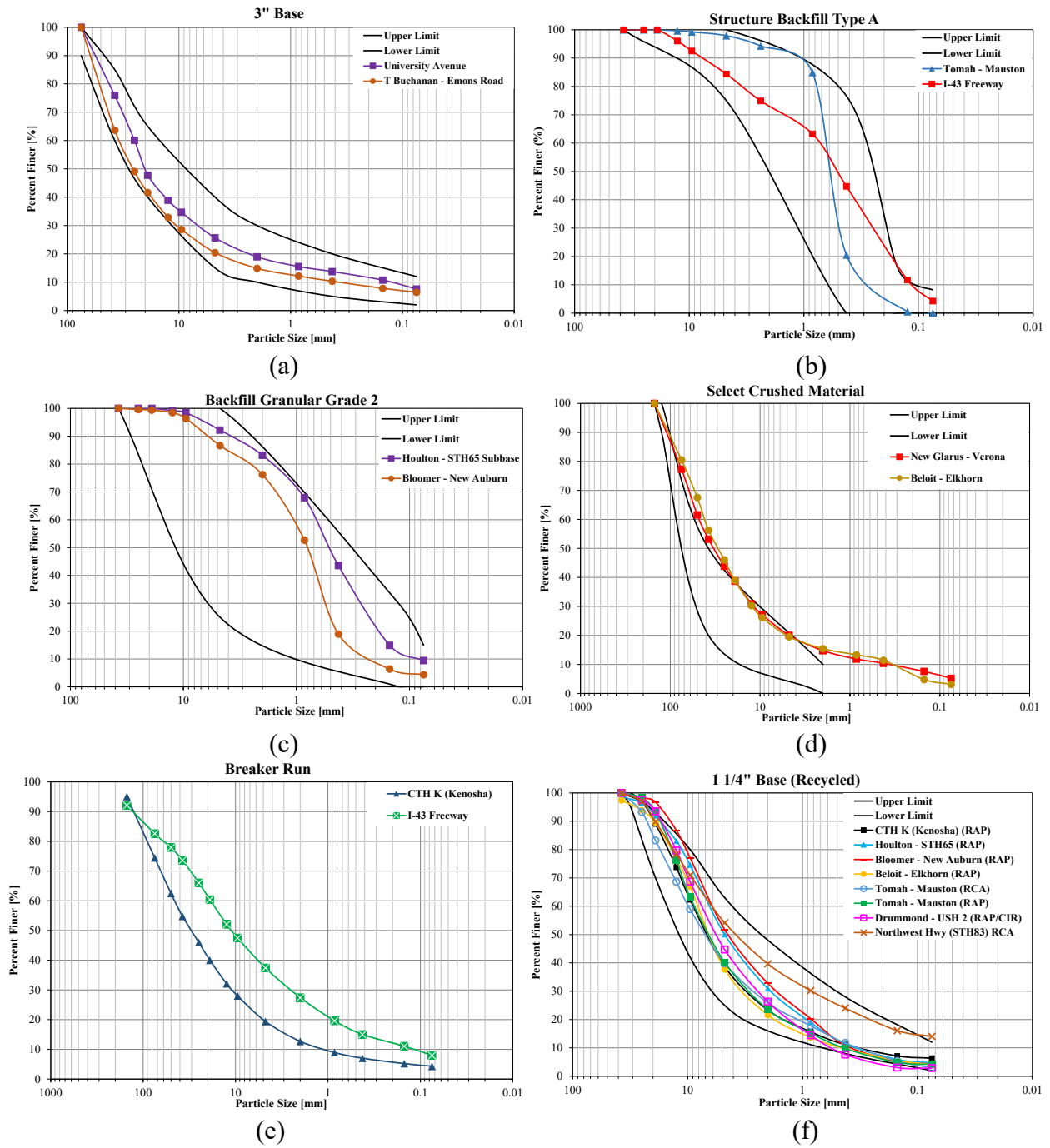
Figure 4.2 Particle size distribution of materials: (a) 3-inch base, (b) structural backfill type a, (c) backfill granular grade 2, (d) select crushed material, (e) breaker run, (f) 1 ¼-inch base (recycled)
