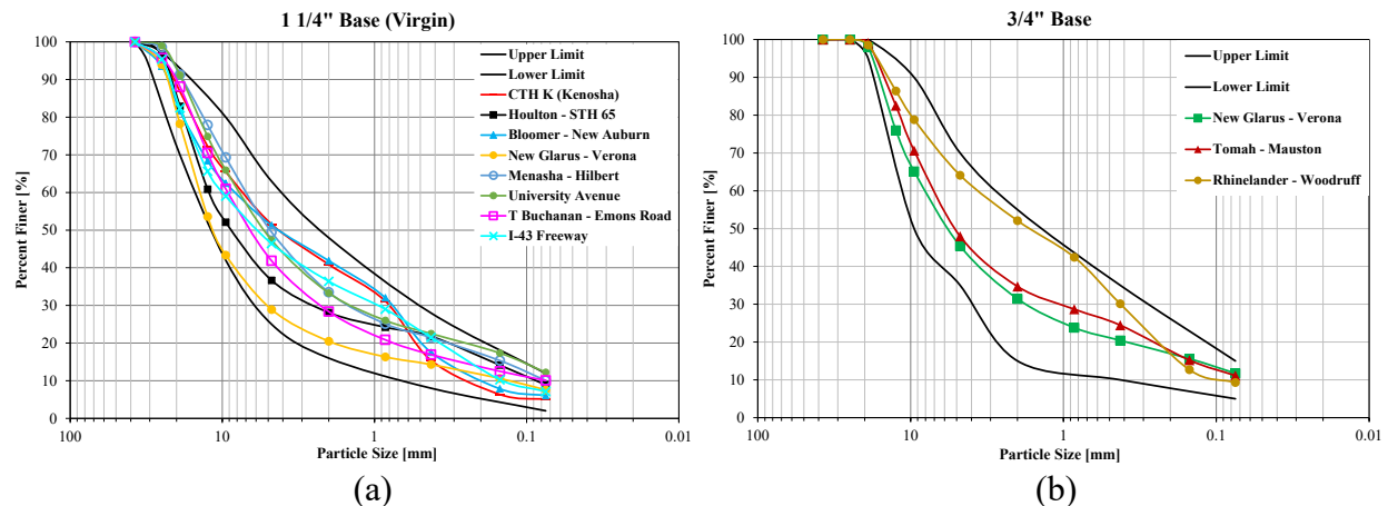
Figure 4.1 Particle size distribution of materials: (a) 1 ¼-inch base, (b) ¾-inch base
