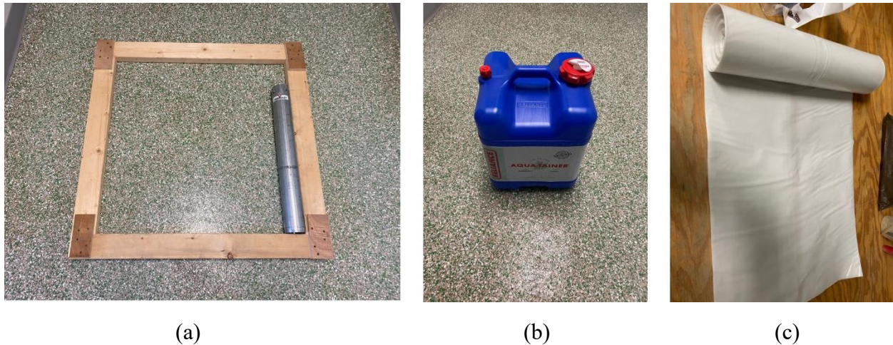
Figure 3.11 (a) 30” x 30” frame, (b) water Container, and (c) 6 mil thick liner
